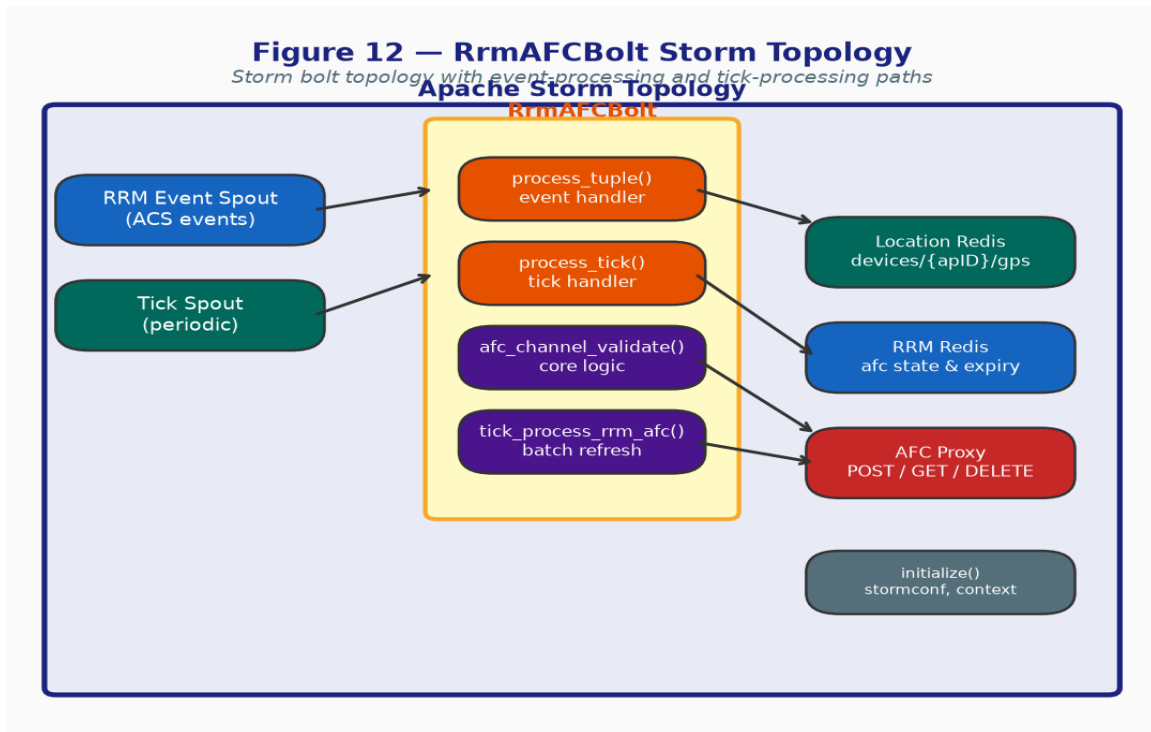
Figure 12 — RrmAFCBolt Storm Topology
