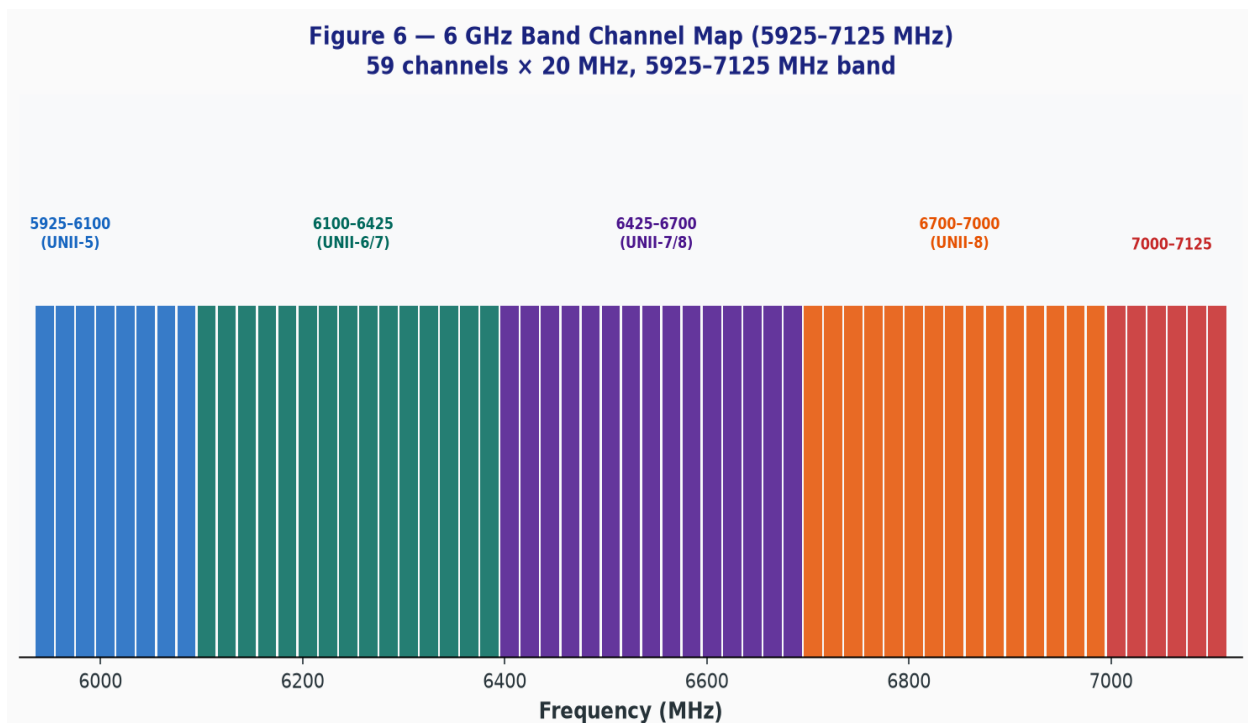
Figure 6 — 6 GHz Band Channel Map (5925–7125 MHz)
