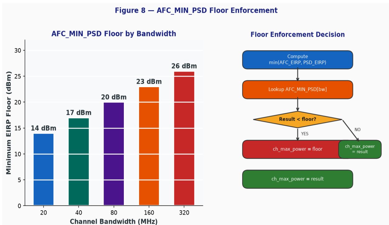
Figure 8 — AFC_MIN_PSD Floor Enforcement Decision
