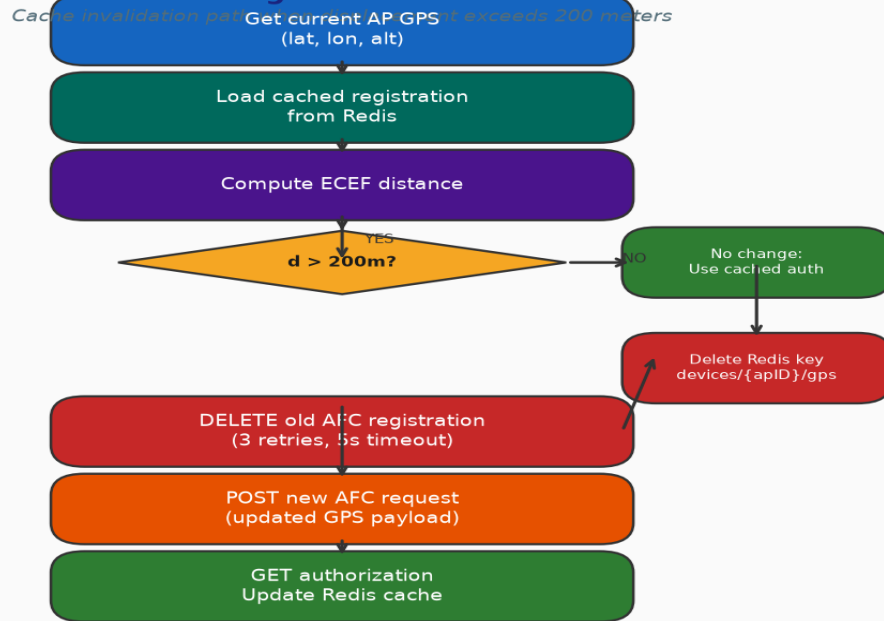
Figure 11 — Location Change Detection and Cache Invalidation
