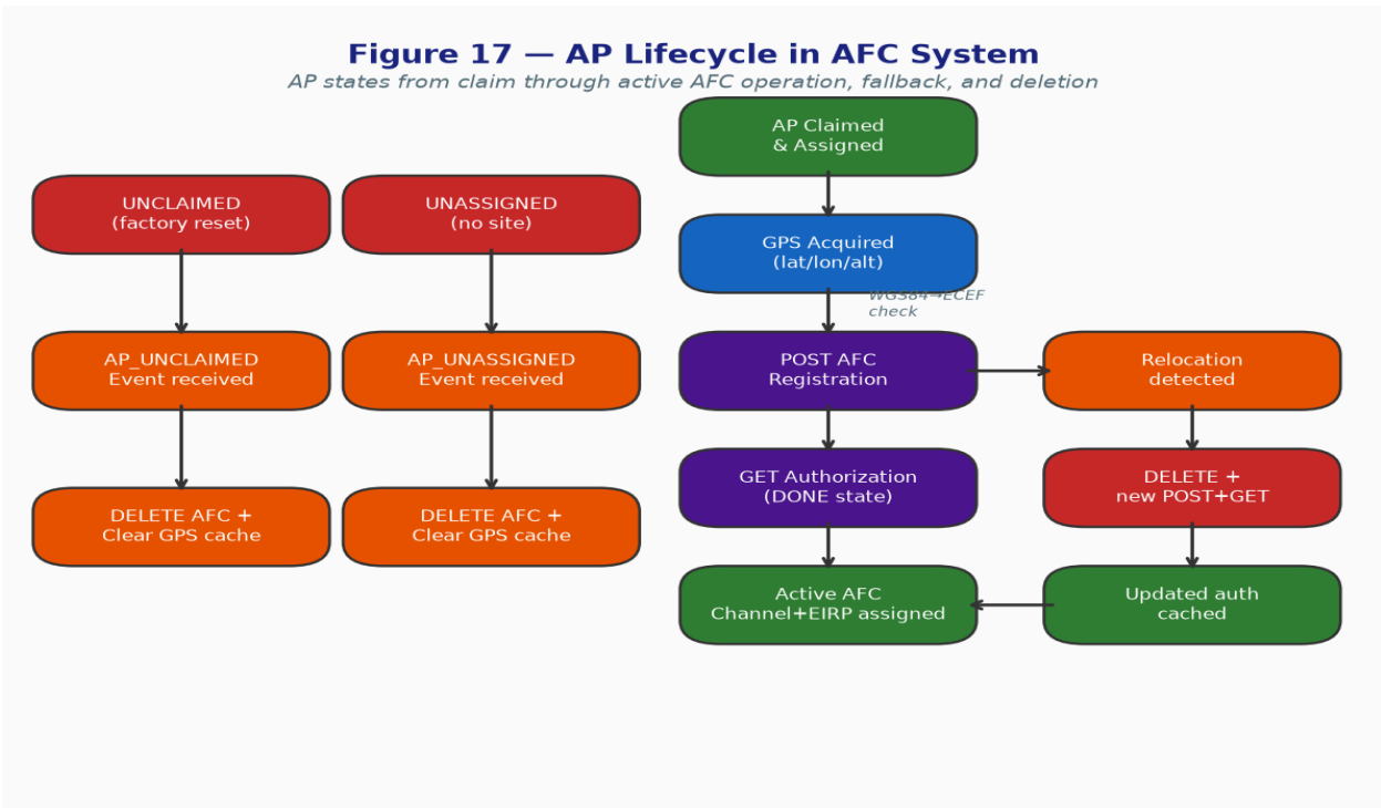
Figure 17 — AP Lifecycle in AFC System
