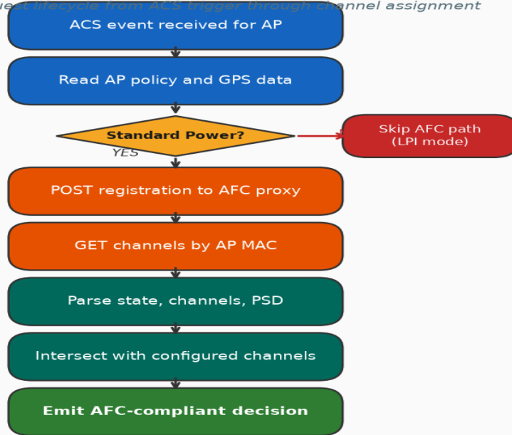
Figure 2 — AFC Request Lifecycle Flowchart End-to-end request lifecycle from ACS trigger through channel assignment
