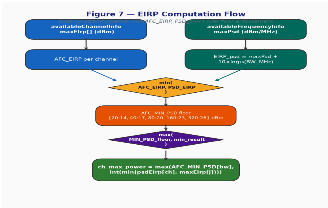
Figure 7 — EIRP Computation Flow
