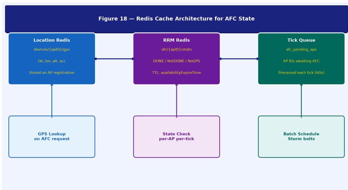
Figure 18 — Redis Cache Architecture for AFC State
