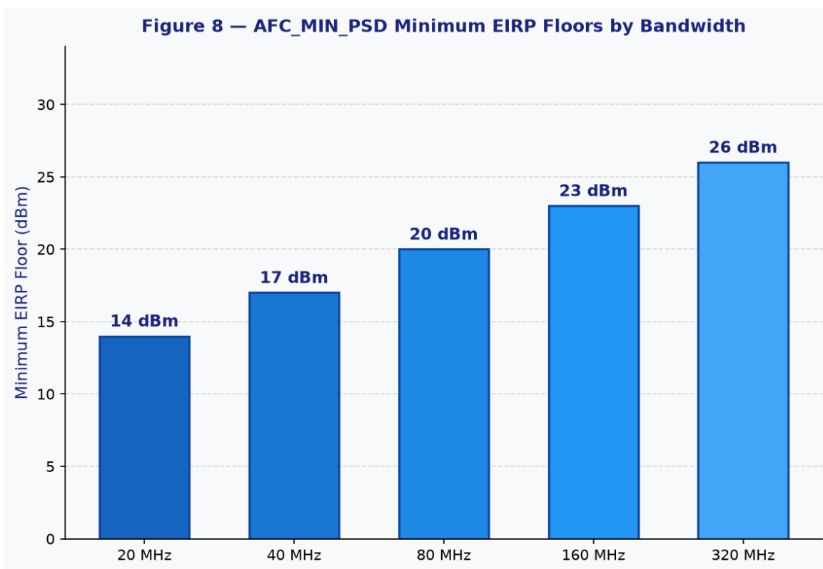
Figure 8 — AFC_MIN_PSD Minimum EIRP Floors by Bandwidth
