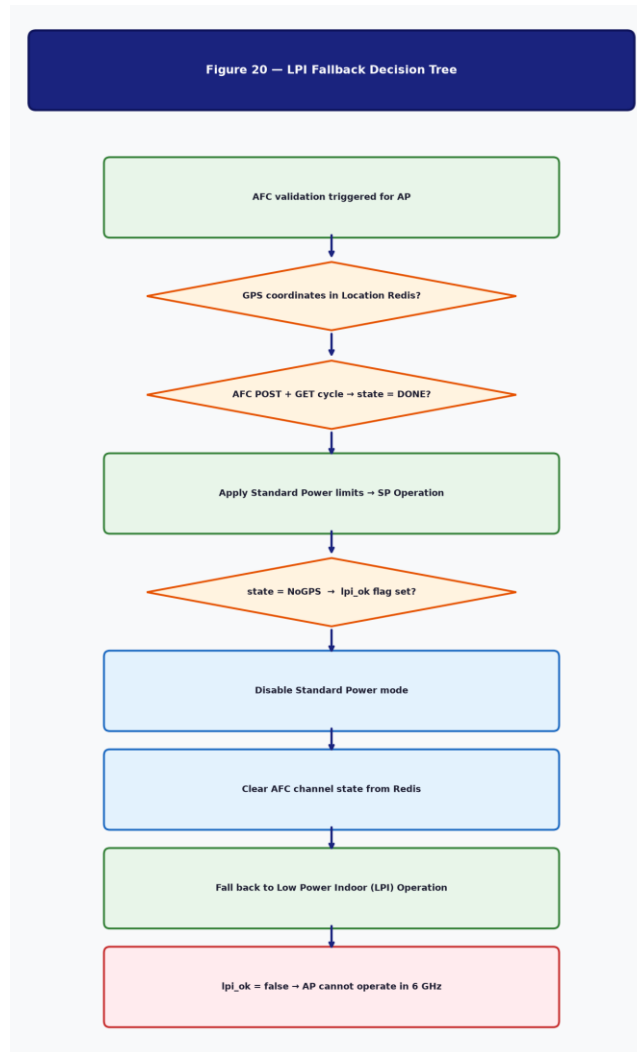
Figure 20 — LPI Fallback Decision Tree
