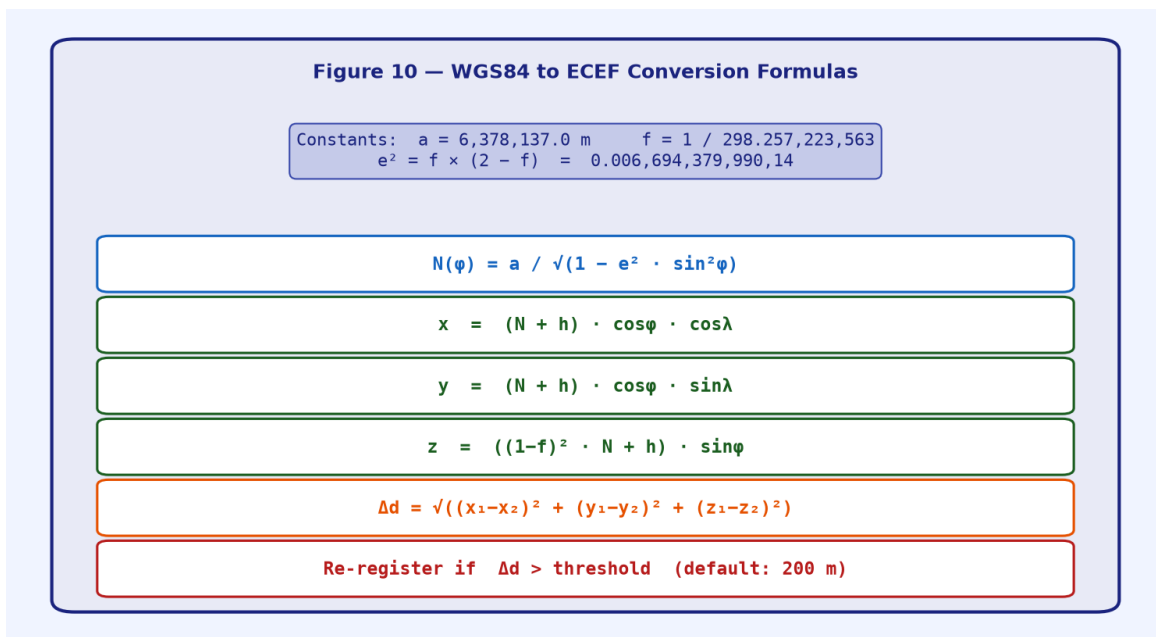
Figure 10 — WGS84 to ECEF Conversion Formula Block
