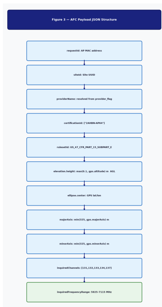
Figure 3 — AFC Payload JSON Structure
