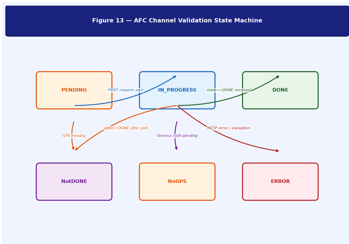
Figure 13 — AFC Channel Validation State Machine
