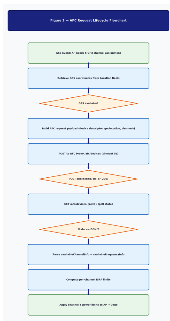
Figure 2 — AFC Request Lifecycle Flowchart
