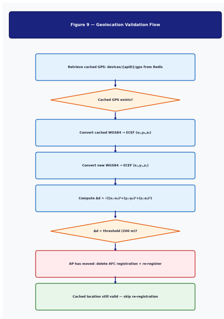
Figure 9 — Geolocation Validation Flow
