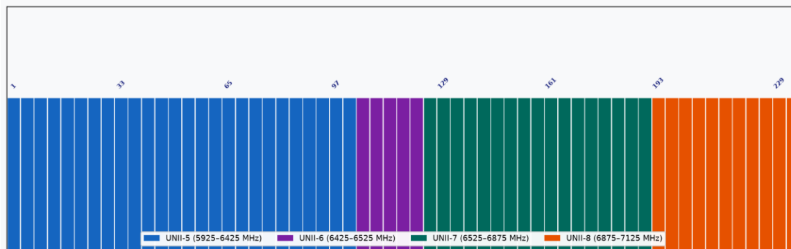
Figure 6 — 6 GHz Band Channel Map (5925–7125 MHz)
