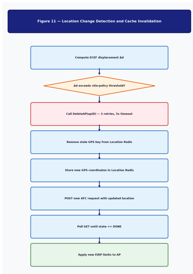
Figure 11 — Location Change Detection and Cache Invalidation
