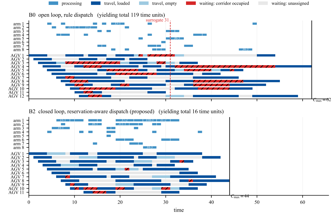
Fig. 8. B0 (top) and B2 (bottom) on the same funnel instance. Robotic arms and vehicles share the time axis; vehicle rows distinguish empty and loaded legs, and two kinds of gap. A gap between the two legs of the same transport task: the vehicle is held at a berth by an occupied corridor, i.e. yielding wait, the delay this paper treats. A gap between different tasks: the vehicle has nothing to do. The two are coloured separately, so that idle time is not read as yielding wait.
