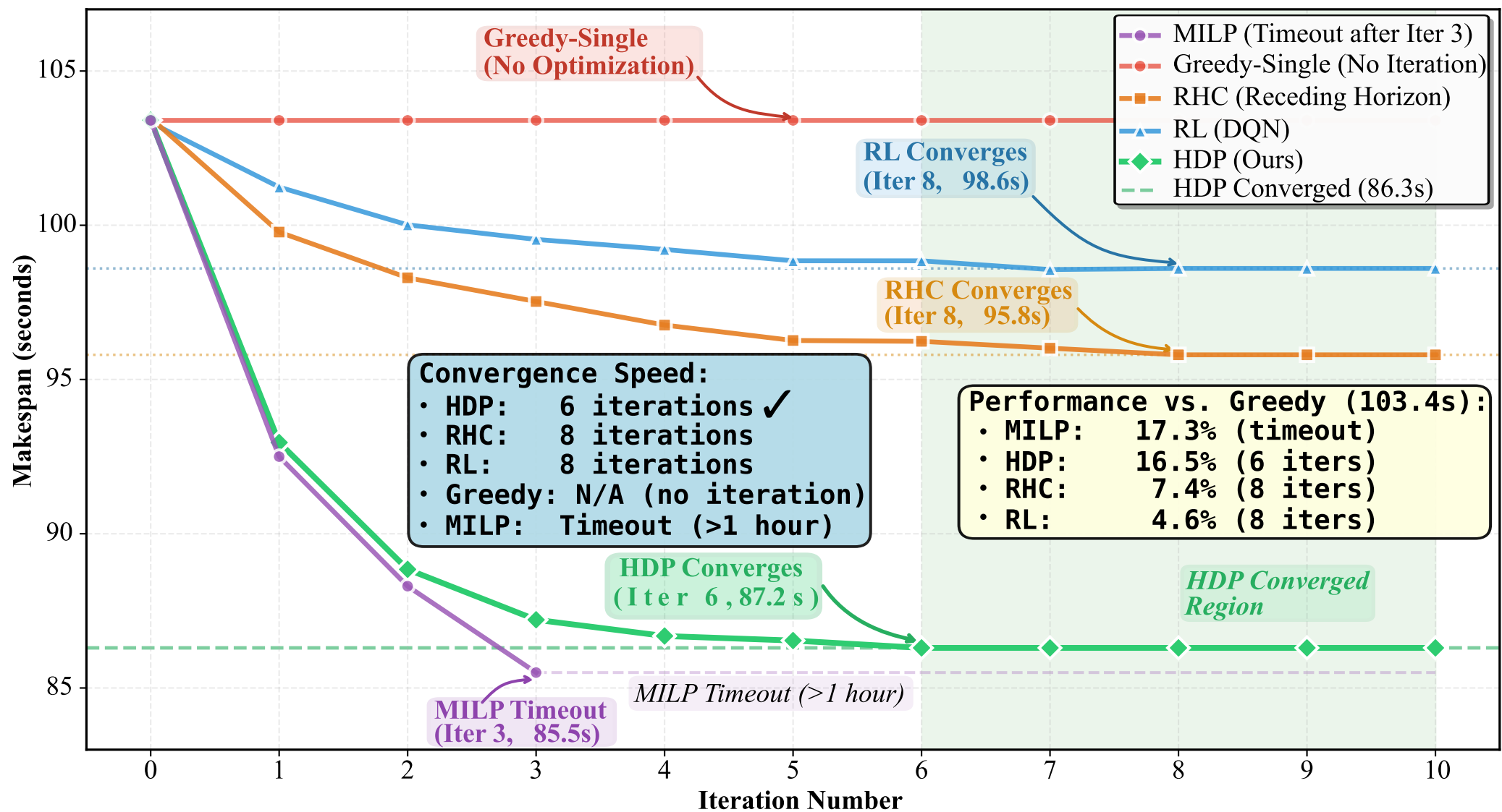
Convergence Behavior of HDP vs. Baselines on DS2 (30 Tasks)
