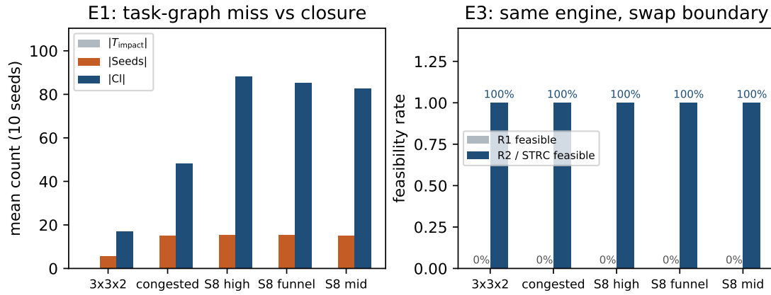
Fig. 5. Visualization of the extended E1/E3 results (means over 5 instances \times 10 random seeds). Left: the affected set on the operation-precedence graph is empty, whereas the seed set and the reservation impact set are nonempty. Bar heights are means over the 10 cells of each instance; dispersion as IQR is given in Table 4 (the per-instance IQR of |CI| lies between 2 and 8; the affected-set group is always zero and thus has no dispersion). Right: with the same rerouting and only the scope object replaced, the feasibility rate is 0 for R1 and 100% for R2; this panel shows cell-wise counts (50 cells each), so no dispersion is given.
