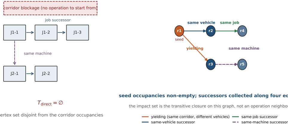
Fig. 2. The vertex sets of the two graphs are disjoint (schematic construction). (a) Operation-precedence graph G_T : vertices are operations, and a corridor blockage finds no seed operation. (b) Reservation dependency graph G_R : vertices are corridor occupancies; starting from the occupancies overlapping the blockage window, subsequent occupancies are included along the four kinds of dependency edges (yielding, same vehicle, same job, same machine; Definition 4).
