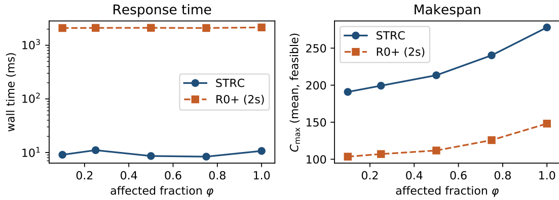
Fig. 9. Sweep over disturbance magnitude (congested_8x4x4, 10 random seeds): runtime (log scale) and makespan of bounded repair and R0+ as functions of \phi . Curves show per-level means; dispersion is measured as in Table 12 (interquartile range). On the runtime side, the range over the whole sweep is 2.2–23.8 ms, always on the order of ten milliseconds; this is the only result on which the conclusion of this section rests.
