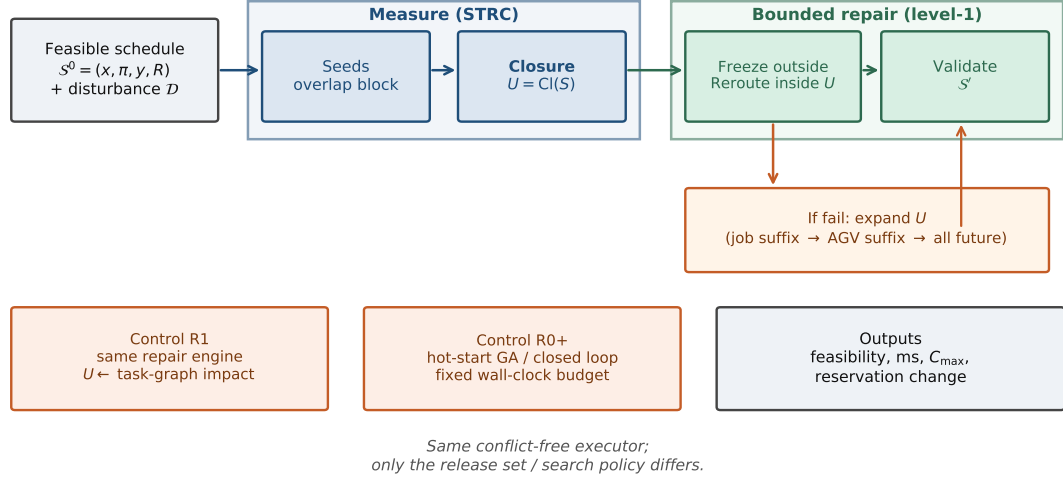
Fig. 4. Bounded repair scoped on the reservation impact set. Top row: the impact set is obtained from the seeds and vehicles are rerouted; middle row: the rewritable scope is escalated after failure; bottom row: the baseline scoping on the operation-precedence graph, the warm-started global rescheduling baseline, and the output metrics. The figure shows only the three method-level paths; three further baselines operate within the millisecond range (Section 6.9).
