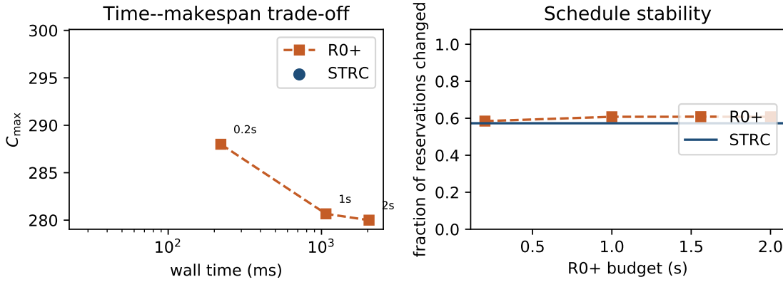
Fig. 7. E5: budget sweep of R0+ (which does not rewrite finished occupancies) versus bounded repair (congested_8x4x4, mean over 3 random seeds). Left: runtime versus C_{\max} ; the two curves do not intersect. Right: occupancy rewrite fraction, about 0.6 for both methods.
