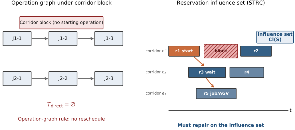
Fig. 1. Motivating example. Left: a corridor blockage makes no operation or machine unexecutable as planned, so the operation-precedence graph contains no seed operation. Right: under the same disturbance, the corridor occupancies that overlap the blockage interval become seeds and grow into a reservation impact set along yielding and succession relations.
