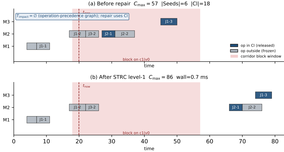
Fig. 6. Case Gantt chart (example_3x3x2, random seed 42). (a) Original schedule before the blockage, colored by membership in CI; (b) after level-1 repair. The affected set on the operation-precedence graph is empty; blue operations are those whose transports in the impact set are rerouted. The figure only illustrates the form of the local change.
