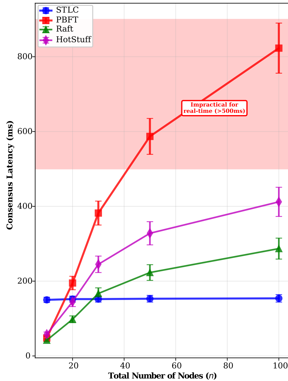
(b) Consensus Latency vs System Size STLC maintains constant latency while PBFT grows with n
