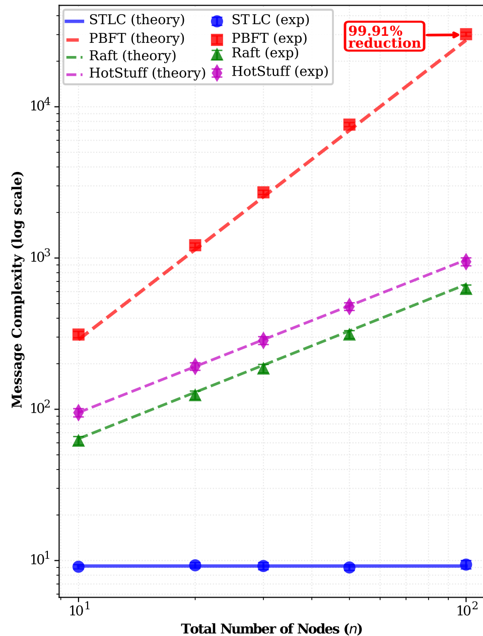
(a) Message Complexity vs System Size STLC maintains O(1) while PBFT scales as O(n^2)
