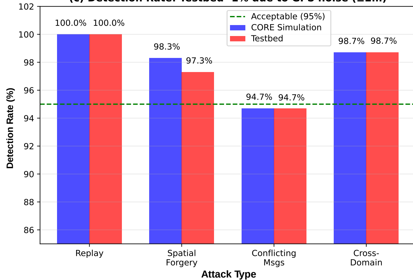
(c) Detection Rate: Testbed -1% due to GPS noise ( \pm 2m )
