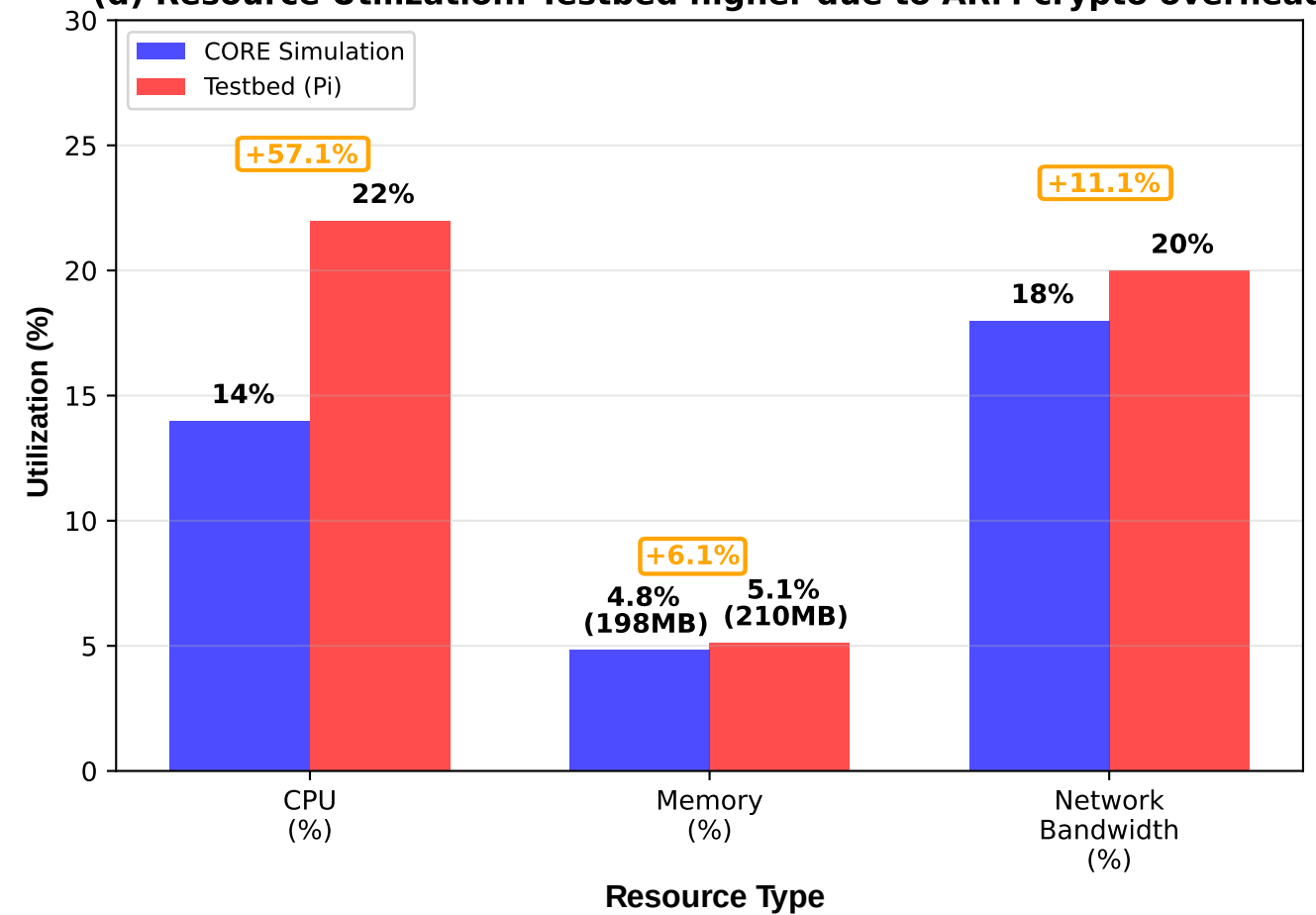
(d) Resource Utilization: Testbed higher due to ARM crypto overhead
