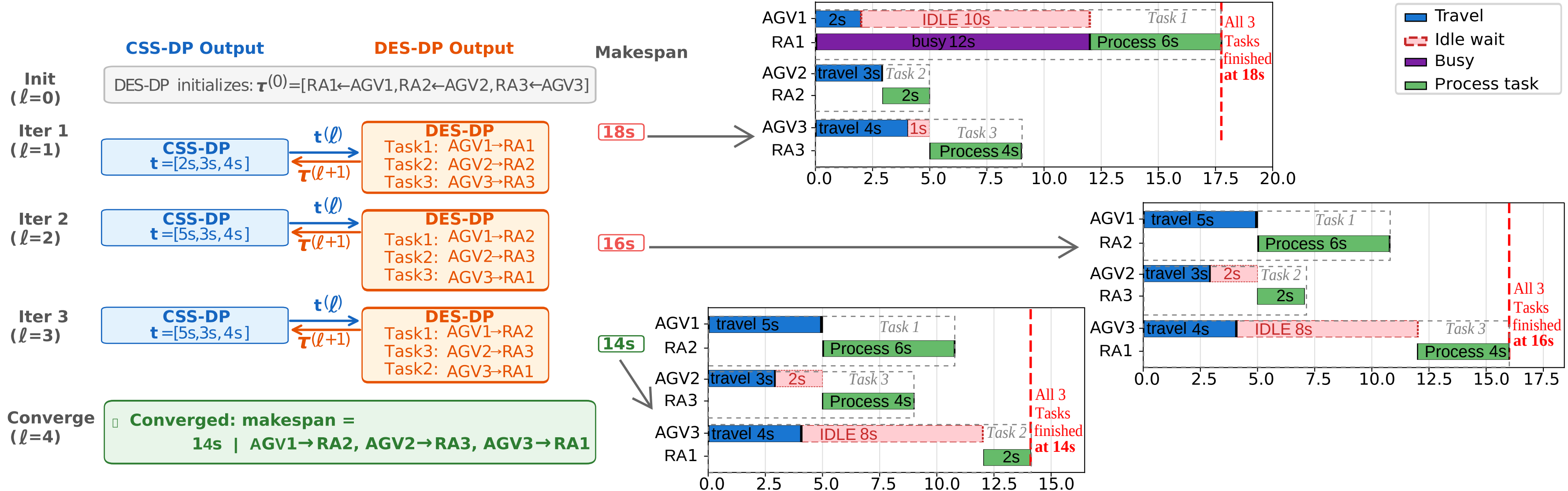
(C) Iterative Coordination: Variable Exchange
