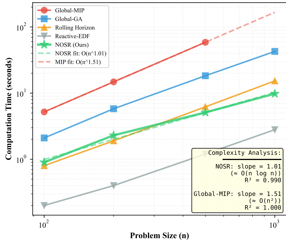
(a) Computation Time vs. Problem Size (Log-log scale)
