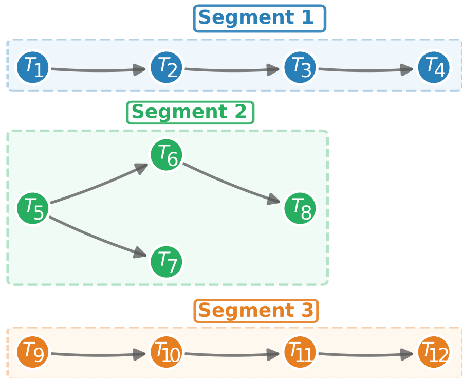
(a) Connected Components ( \rho_{sub} < \rho_0 = 0.3 )
