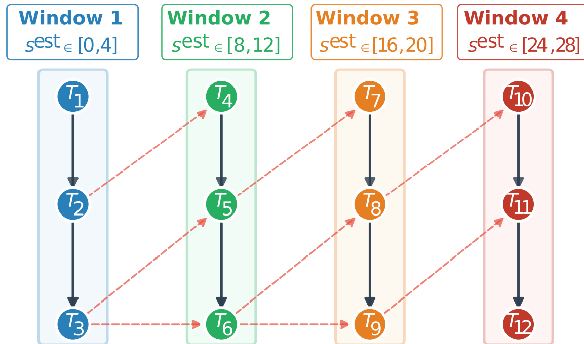
(b) Time-Window Partitioning ( \rho_{sub} \geq \rho_0 = 0.3 )
