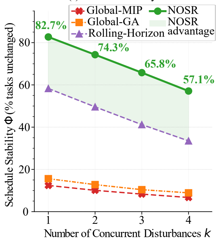
(c) Schedule Stability vs. k
