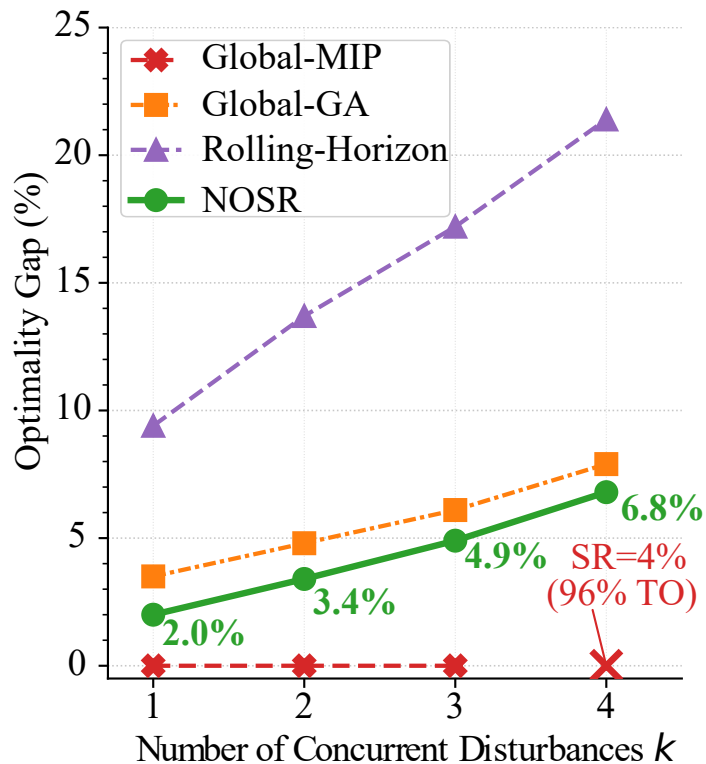
(a) Optimality Gap vs. k
