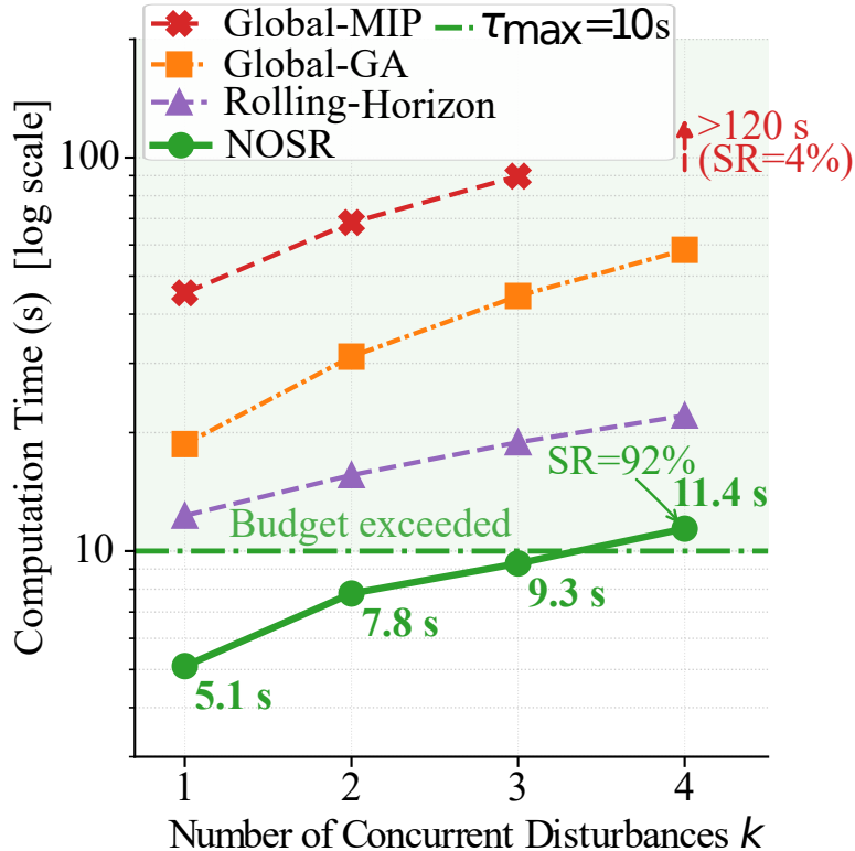
(b) Computation Time vs. k
