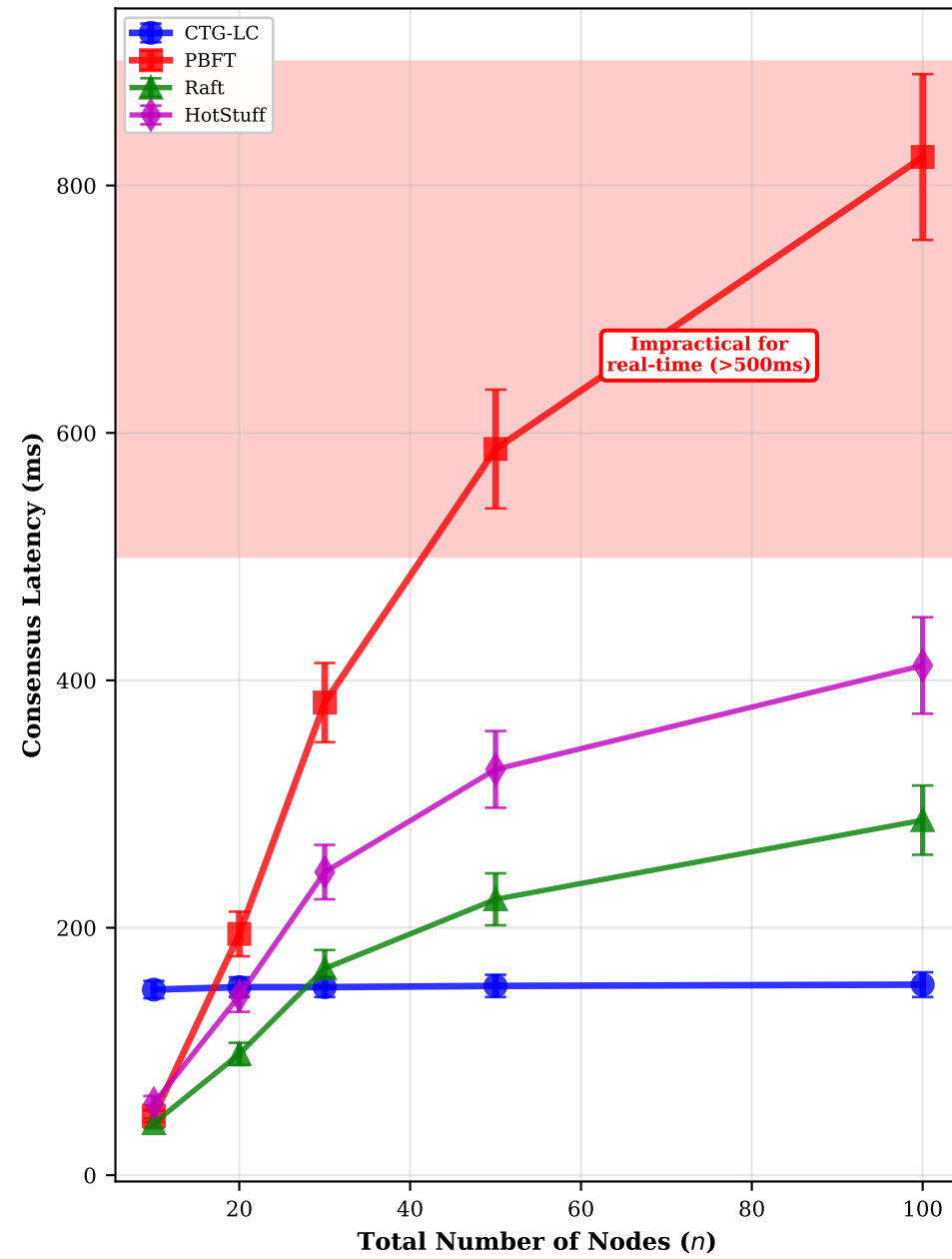
(b) Consensus Latency vs System Size
