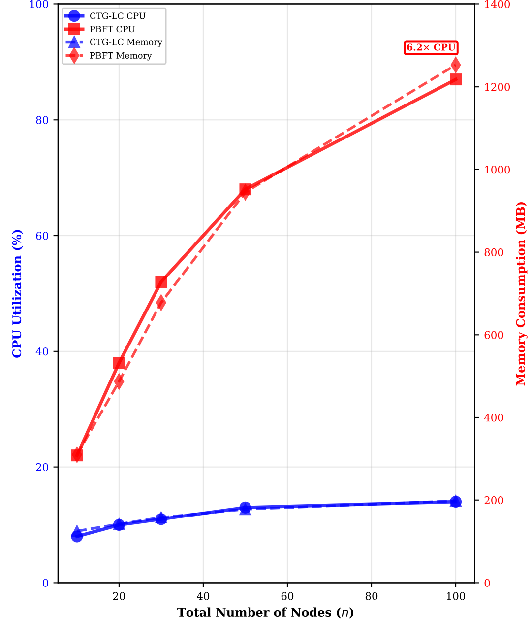
(c) CPU and Memory Overhead
