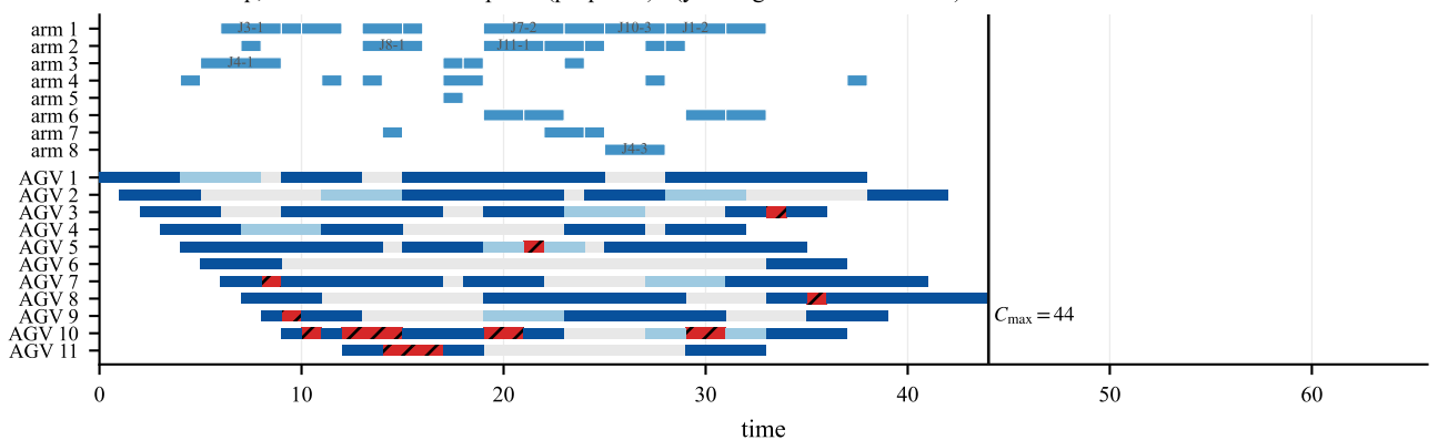
B2 closed loop, reservation-aware dispatch (proposed) (yielding total 16 time units)
