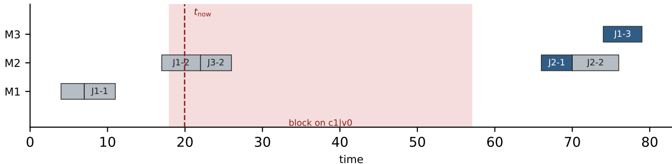
(b) After STRC level-1 C_{\max} = 86 wall=0.5 ms
