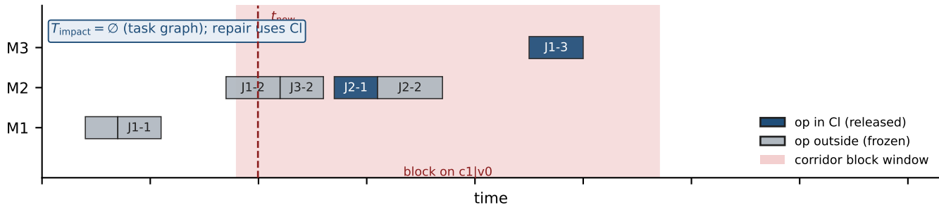
(a) Before repair C_{\max} = 57 |\text{Seeds}|=6 |\text{CI}|=16
