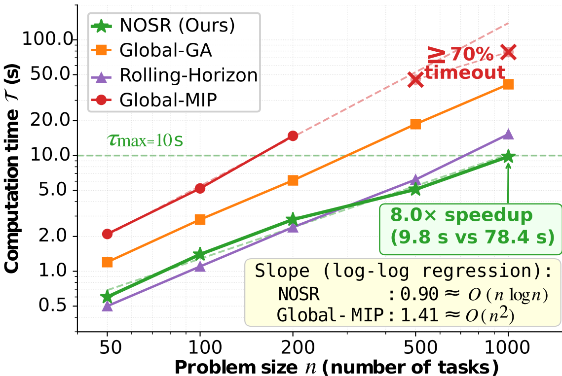
(a) Computation Time vs. Problem Size (log-log scale)
