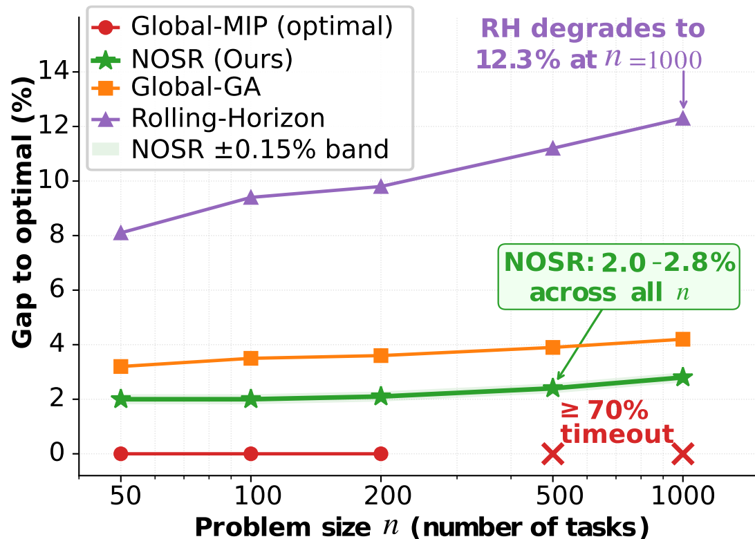
(b) Optimality Gap vs. Problem Size
