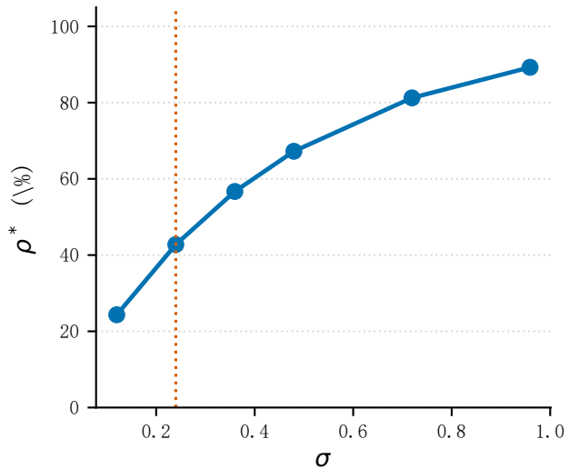
(b) Bound \rho^*(\sigma)
