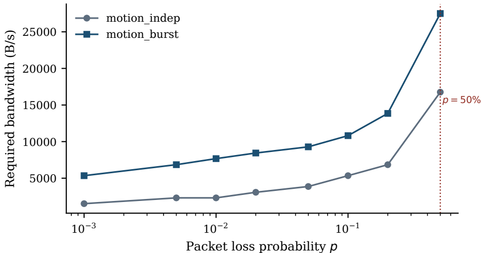
Loss sweep (motion hazard; PISTIS landmark p = 0.5 )
