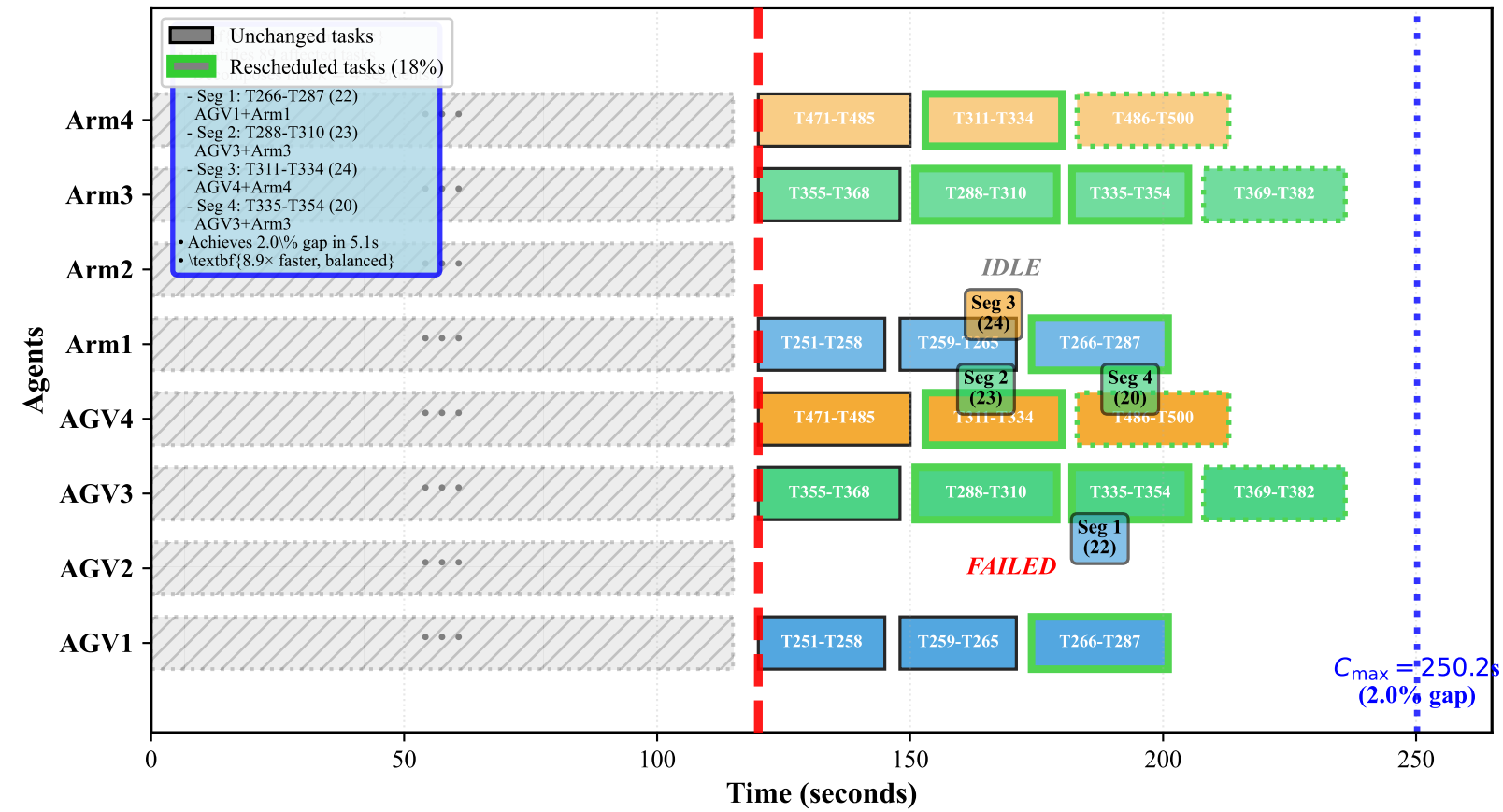
(d) NOSR (Our Approach) Identifies |\mathcal{T}_{\text{aff}}| = 89 tasks (18%), decomposes into k = 4 segments
