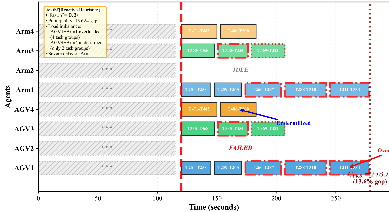
(c) Reactive Heuristic Fast ( \mathcal{T} = 0.8s ) but poor quality (13.6% gap)
