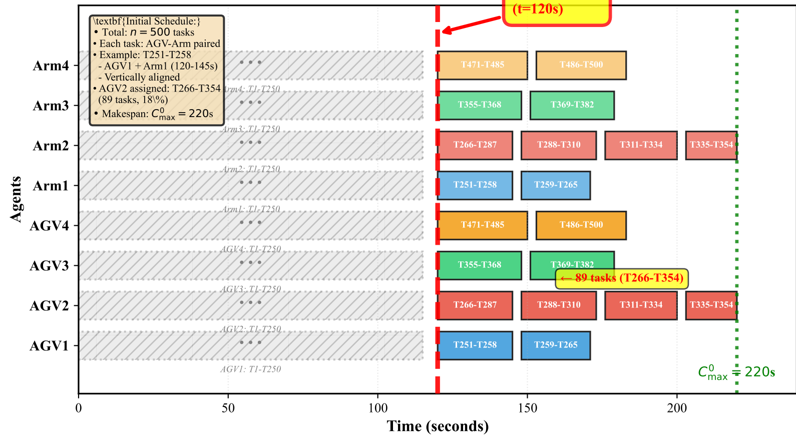
(a) Initial Schedule S_0 AGV2 fails at t=120s, 89 pending tasks need reassignment
