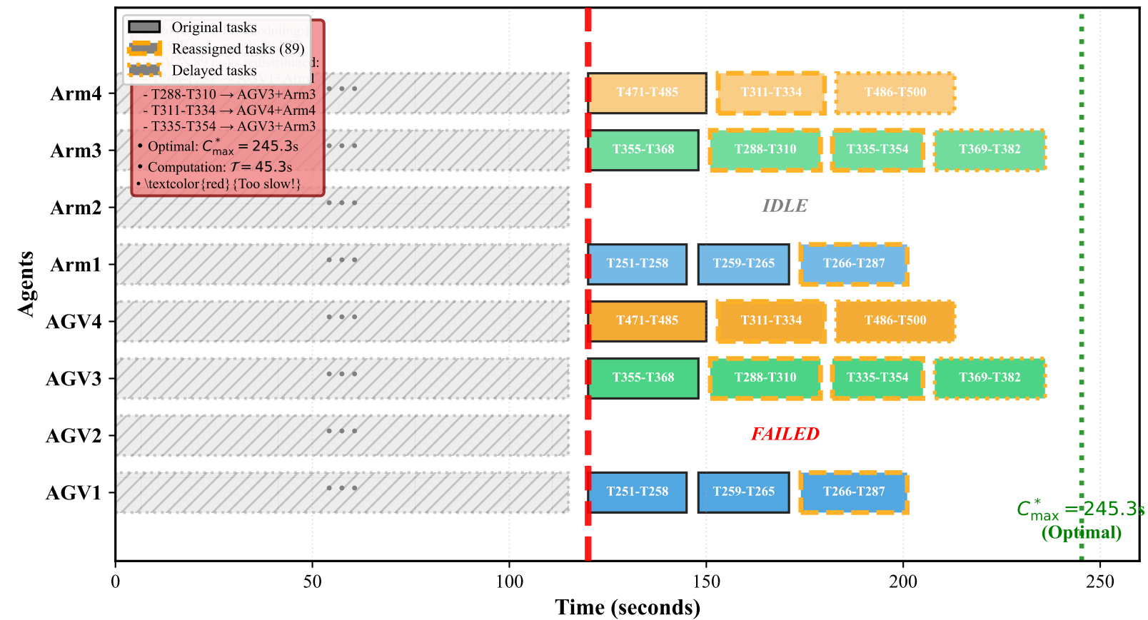
(b) Global Rescheduling Optimal ( C_{\max}^* = 245.3s ) but slow ( \mathcal{T} = 45.3s )
