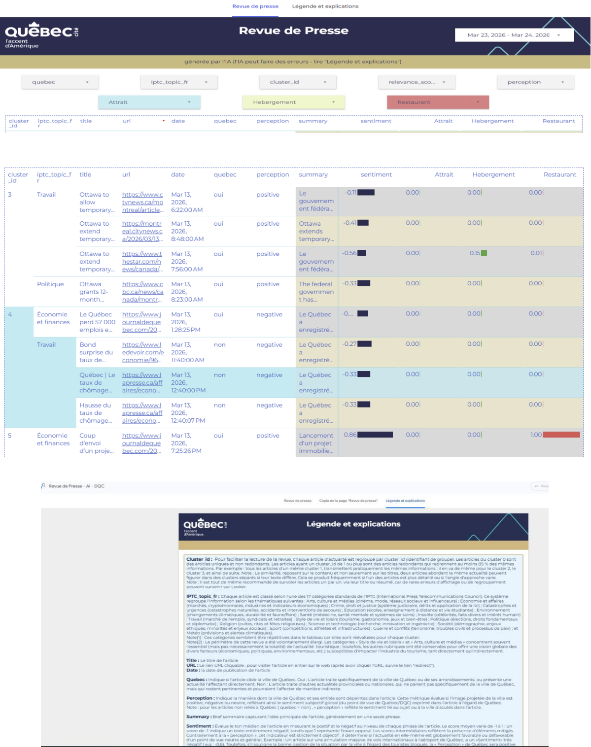
Figure 33: Final DQC Looker dashboard view of clustered articles enriched with sentiment, perception, and domain scores (as well as the dashboard's legend)
