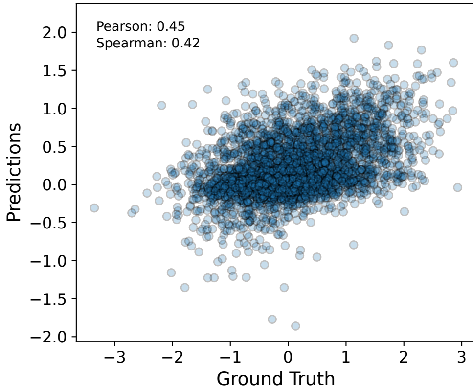
model
