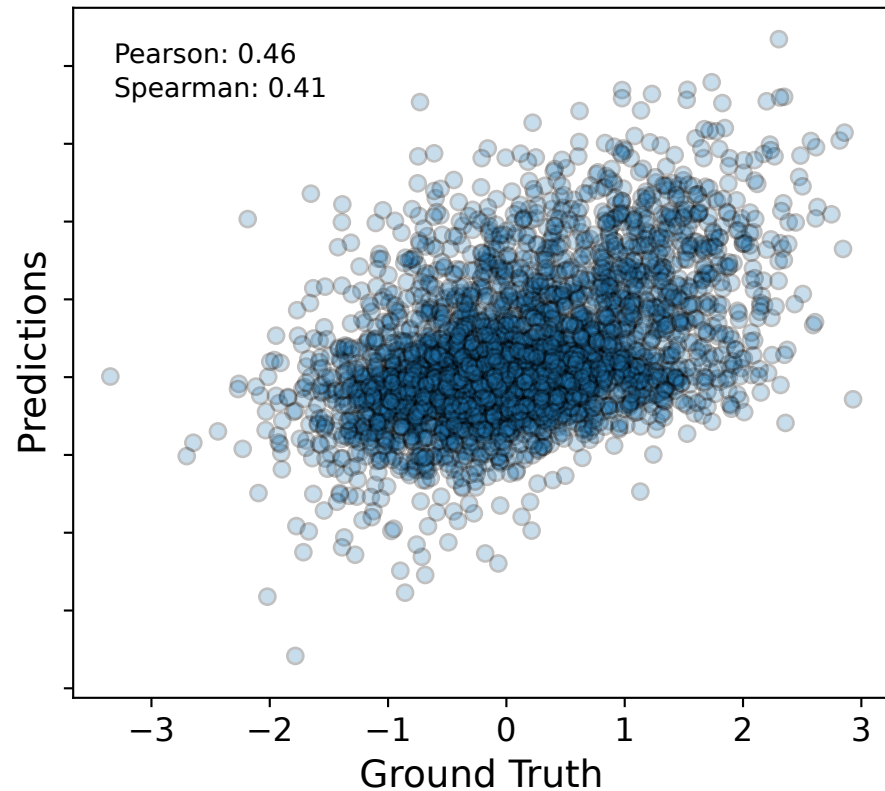
model_ft
