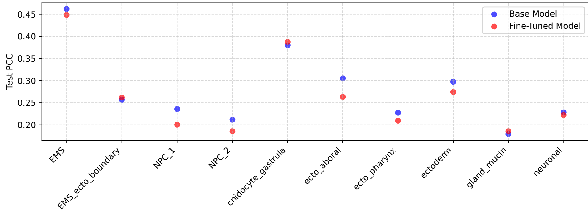
Comparison of Base vs. Fine-Tuned Model PCC per Class
