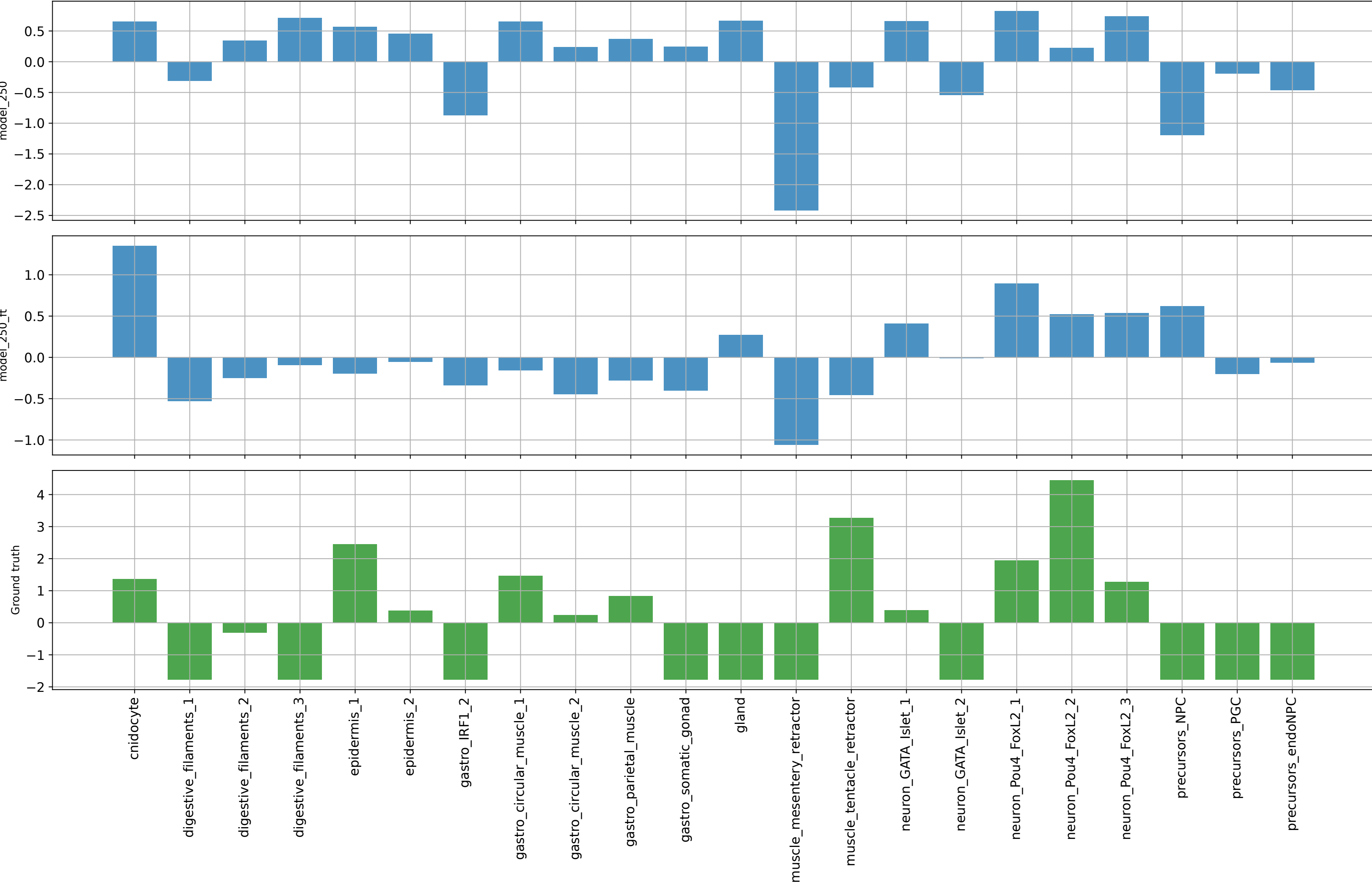
peak89610: NC_064045.1:3438763-3439013 predictions vs ground truth
