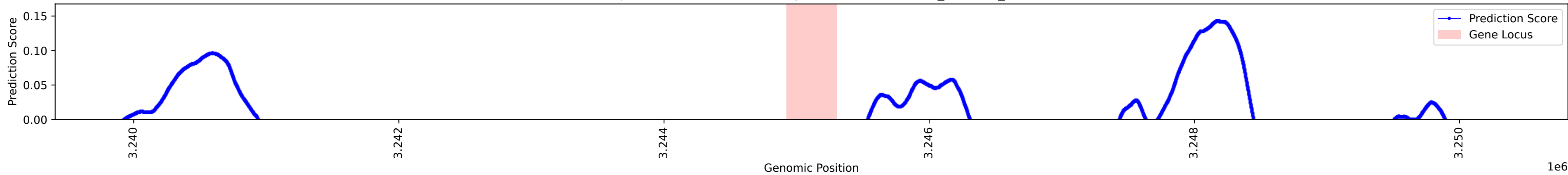
CREsted prediction around Nem64 gene locus for muscle_tentacle_retractor
