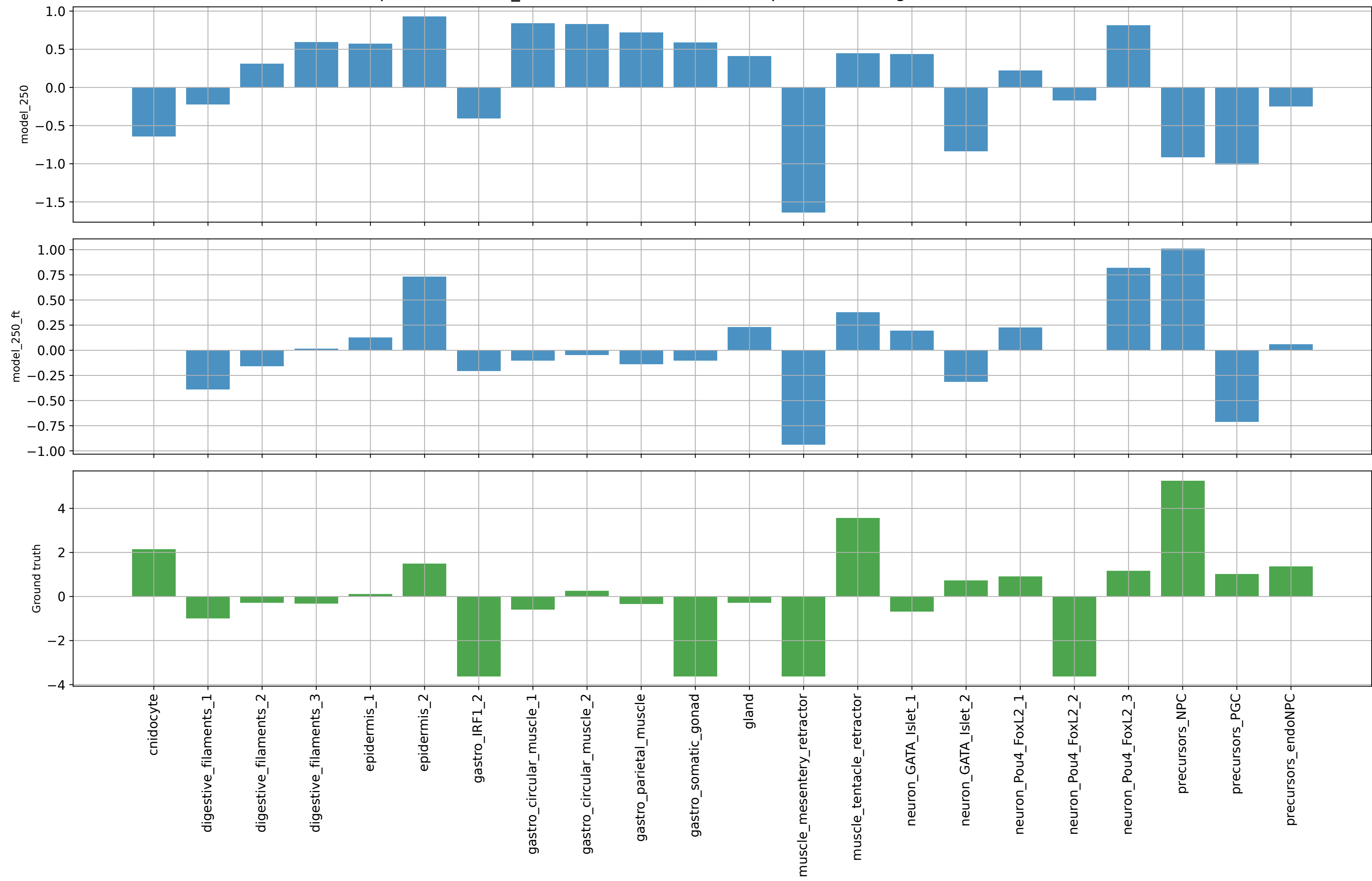
peak11059: NC_064035.1:3247854-3248104 predictions vs ground truth
