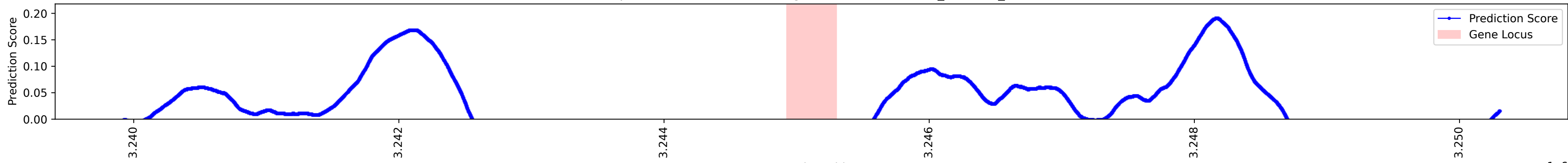
CREsted prediction around Nem64 gene locus for muscle_tentacle_retractor
