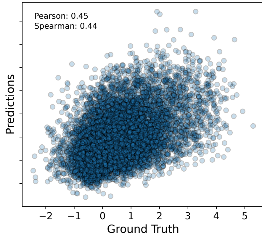
model_500_ft
