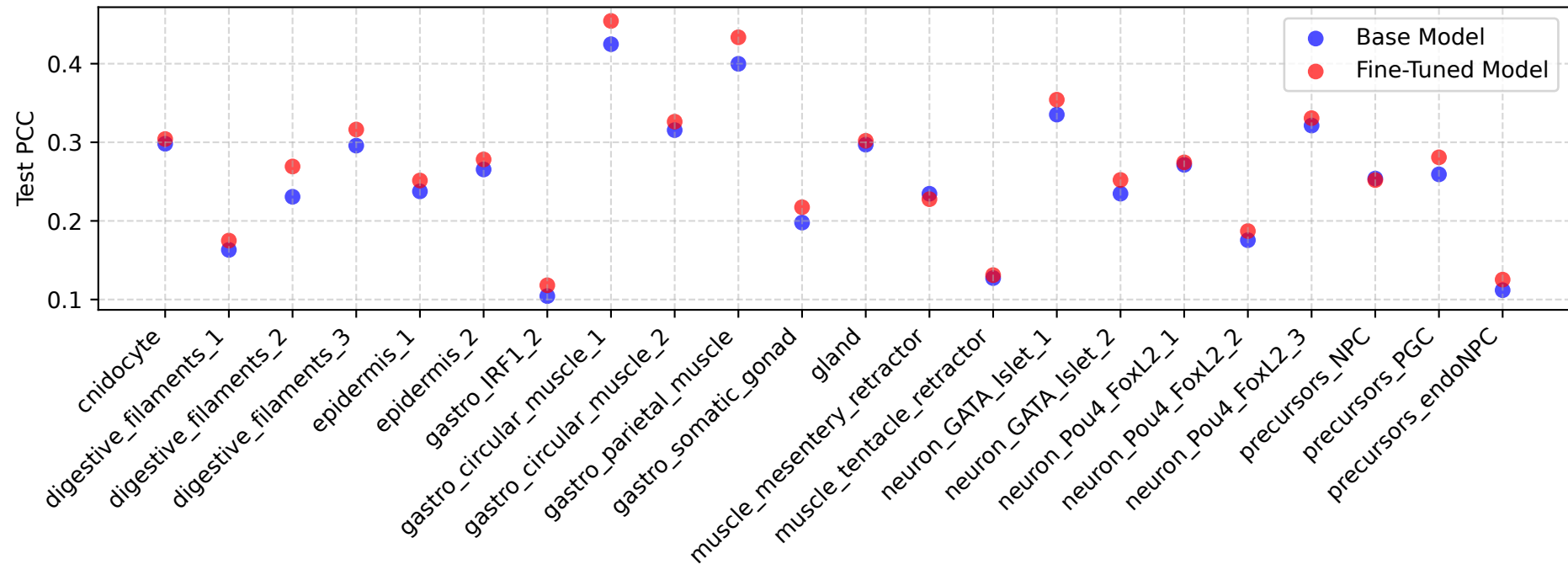
Comparison of Base vs. Fine-Tuned Model PCC per Class
