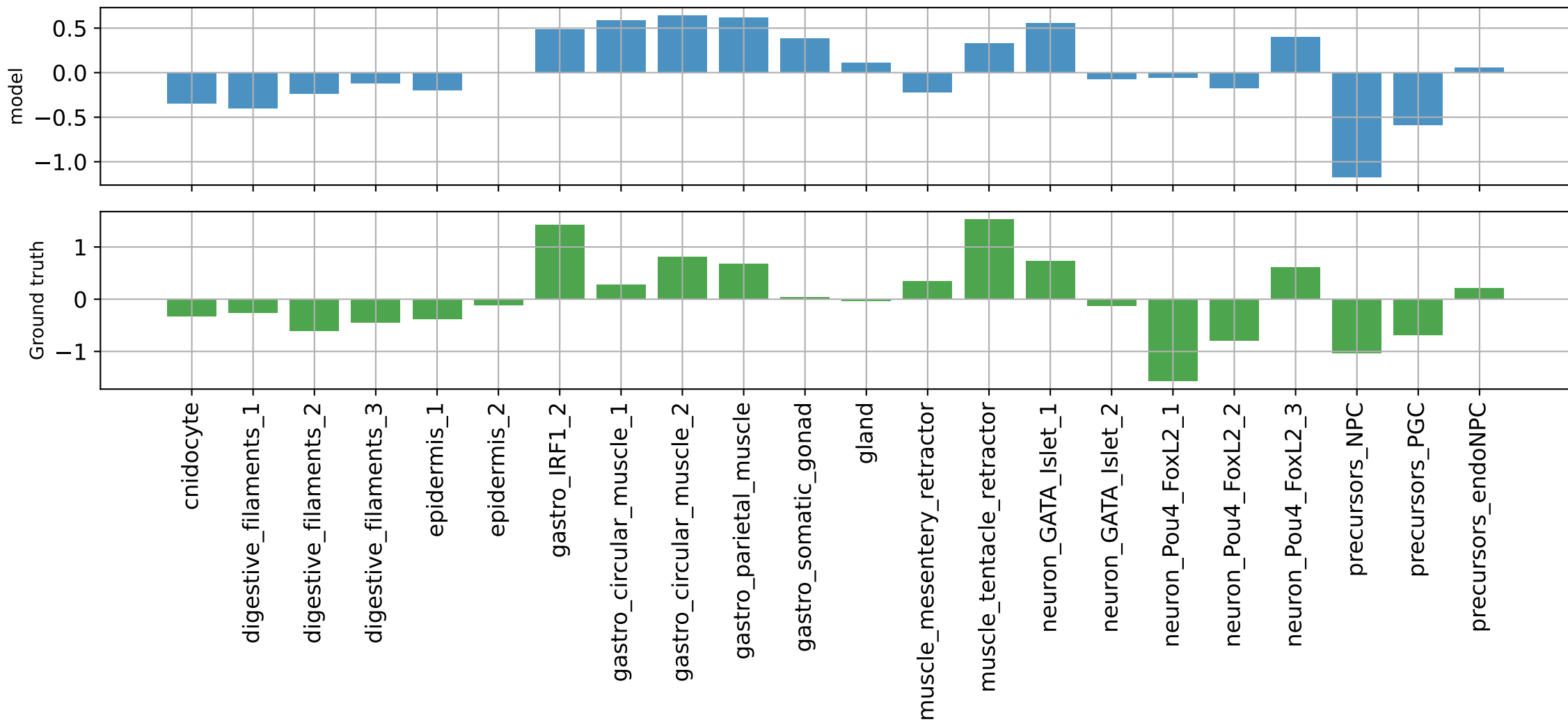
muscle_tentacle_retractor 16: NC_064036.1:3528257-3528757 PCC=0.5244292616844177
