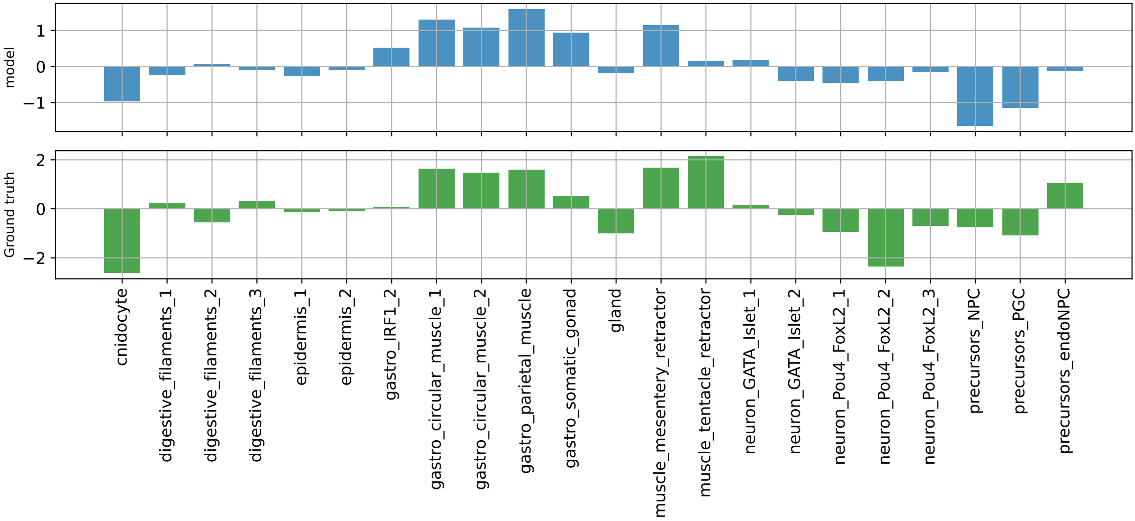
muscle_tentacle_retractor 39: NC_064038.1:10552045-10552545 PCC=0.5220065116882324
