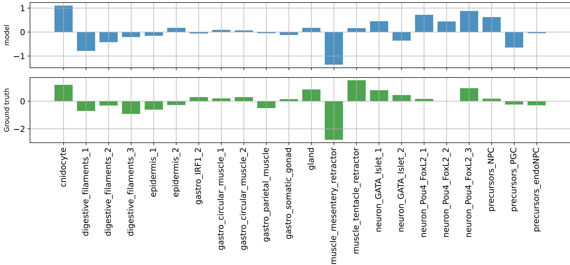
muscle_tentacle_retractor 68: NC_064043.1:5206955-5207455 PCC=0.5463215112686157
