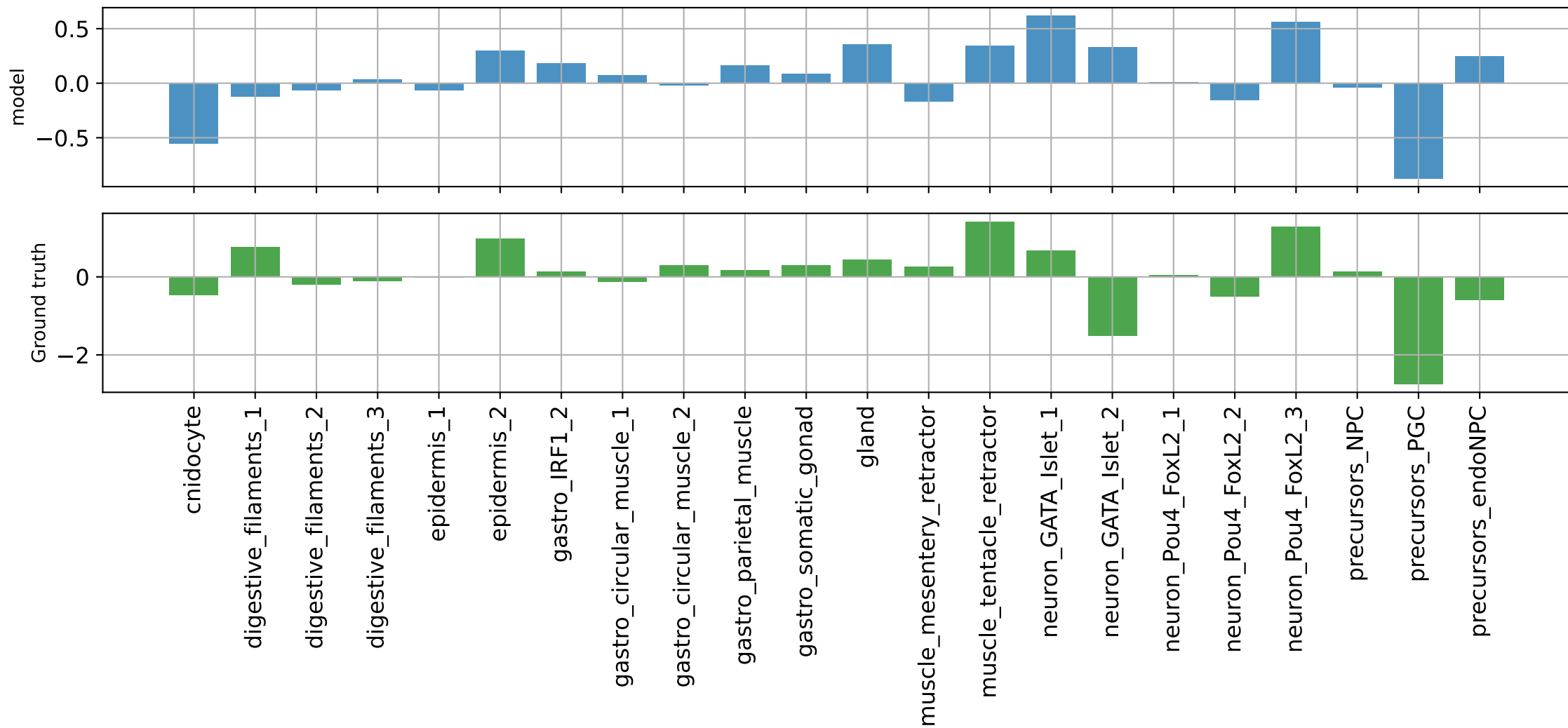
muscle_tentacle_retractor 75: NC_064039.1:3089148-3089648 PCC=0.5169309973716736
