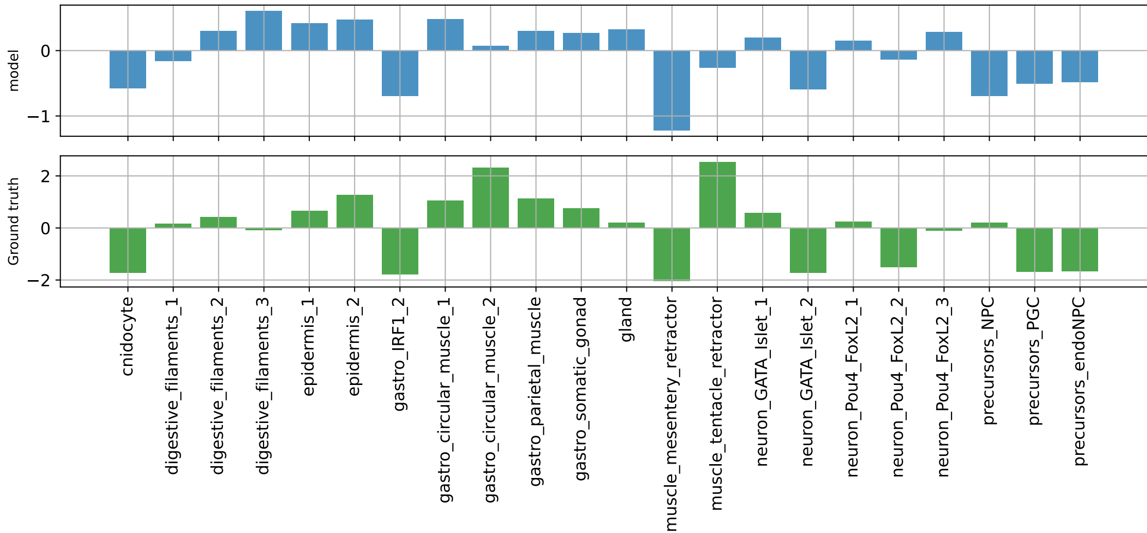
muscle_tentacle_retractor 89: NC_064036.1:5766058-5766558 PCC=0.5166581273078918
