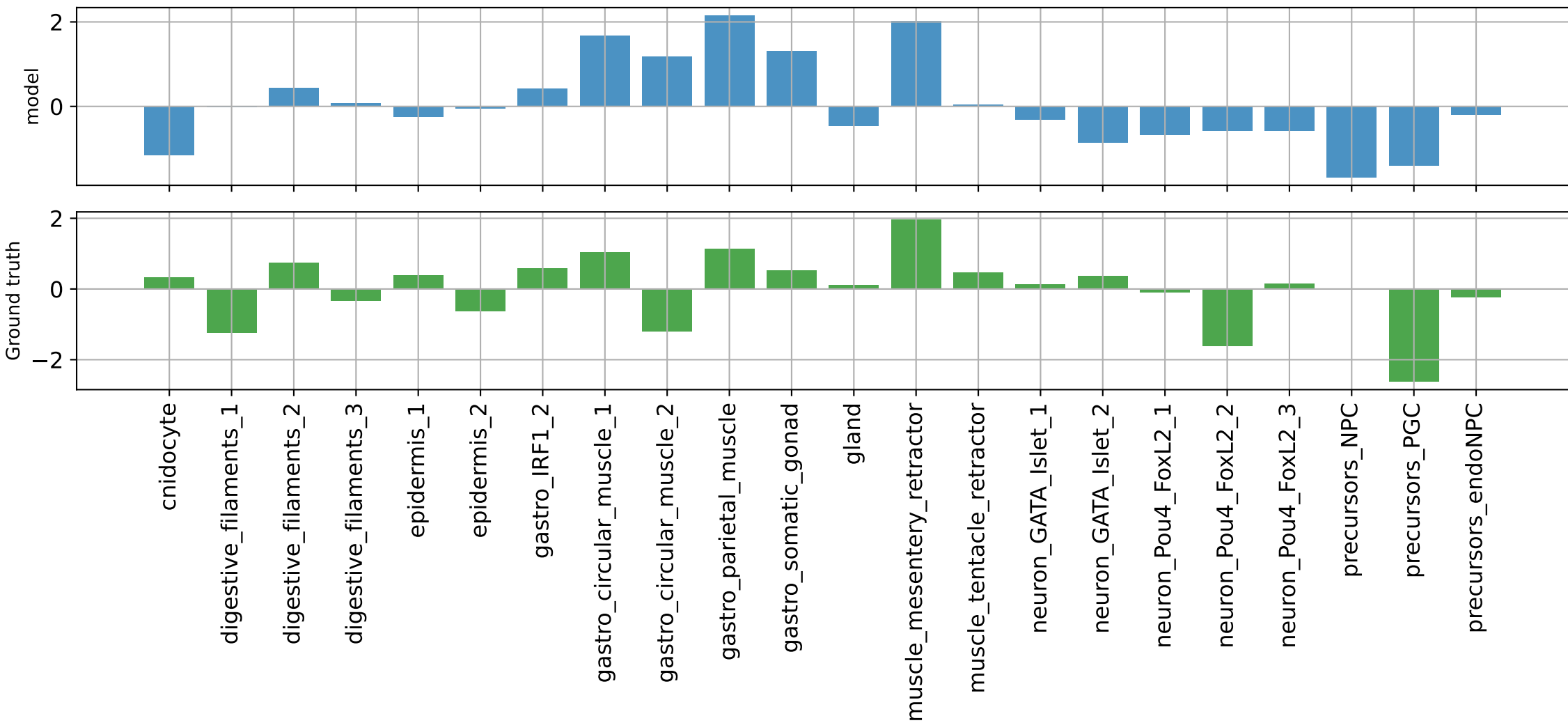
muscle_mesentery_retractor 13: NC_064042.1:518195-518695 PCC=0.5318235754966736
