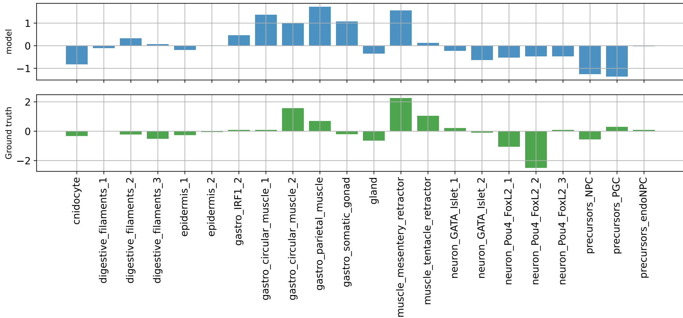
muscle_mesentery_retractor 18: NC_064046.1:1699713-1700213 PCC=0.531046450138092
