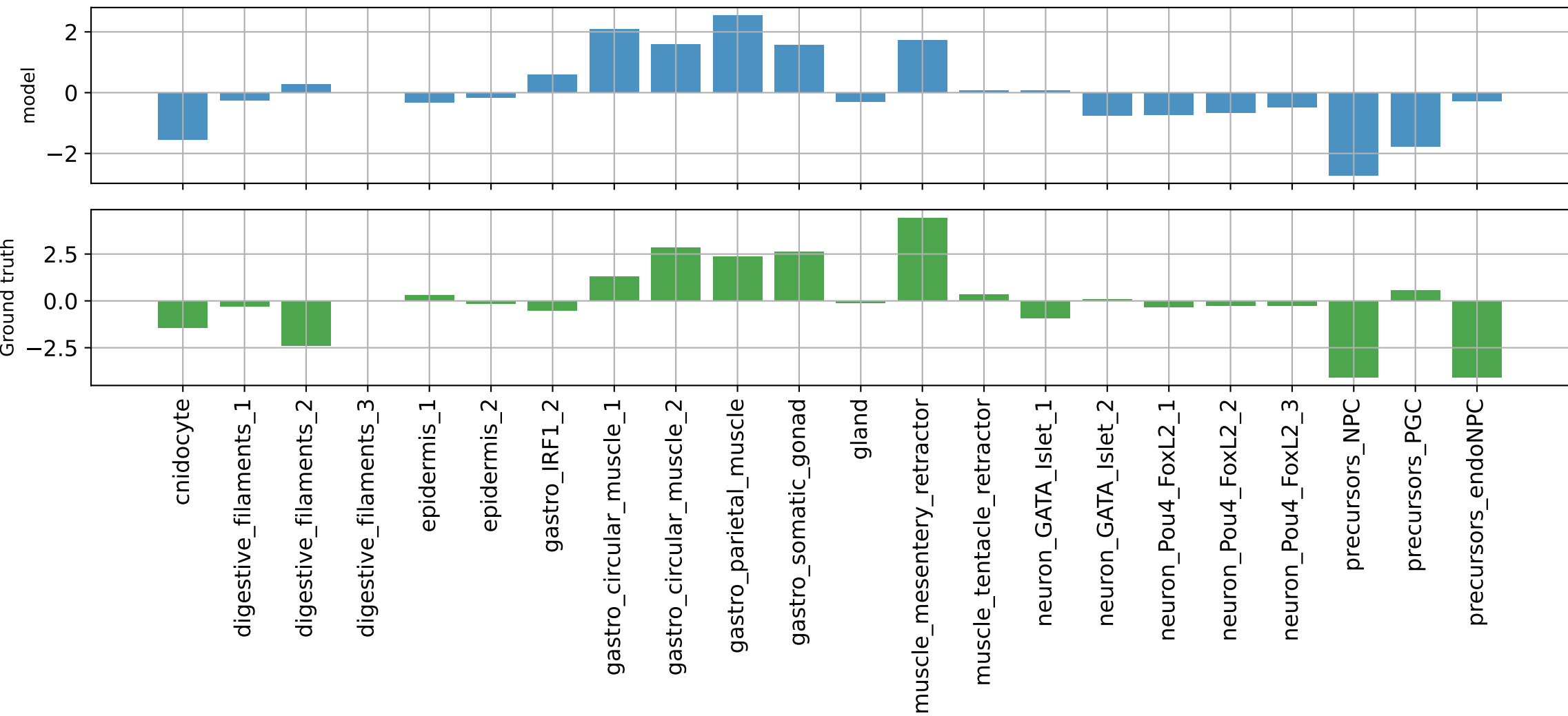
muscle_mesentery_retractor 8: NC_064036.1:17885869-17886369 PCC=0.703463077545166
