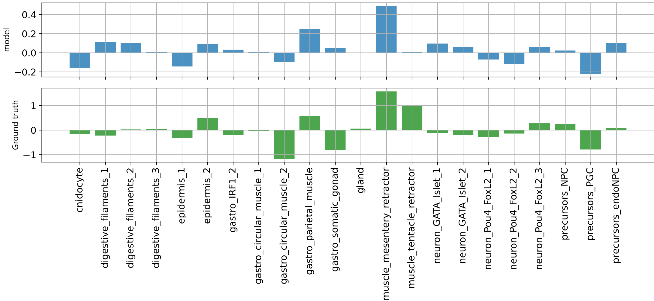
muscle_mesentery_retractor 9: NC_064039.1:11612801-11613301 PCC=0.7041599154472351
