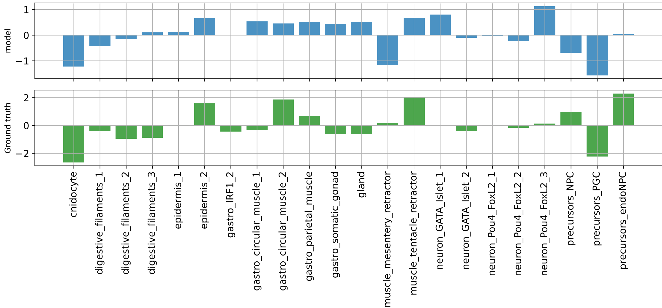
muscle_tentacle_retractor 10: NC_064034.1:7071070-7071570 PCC=0.5176921486854553
