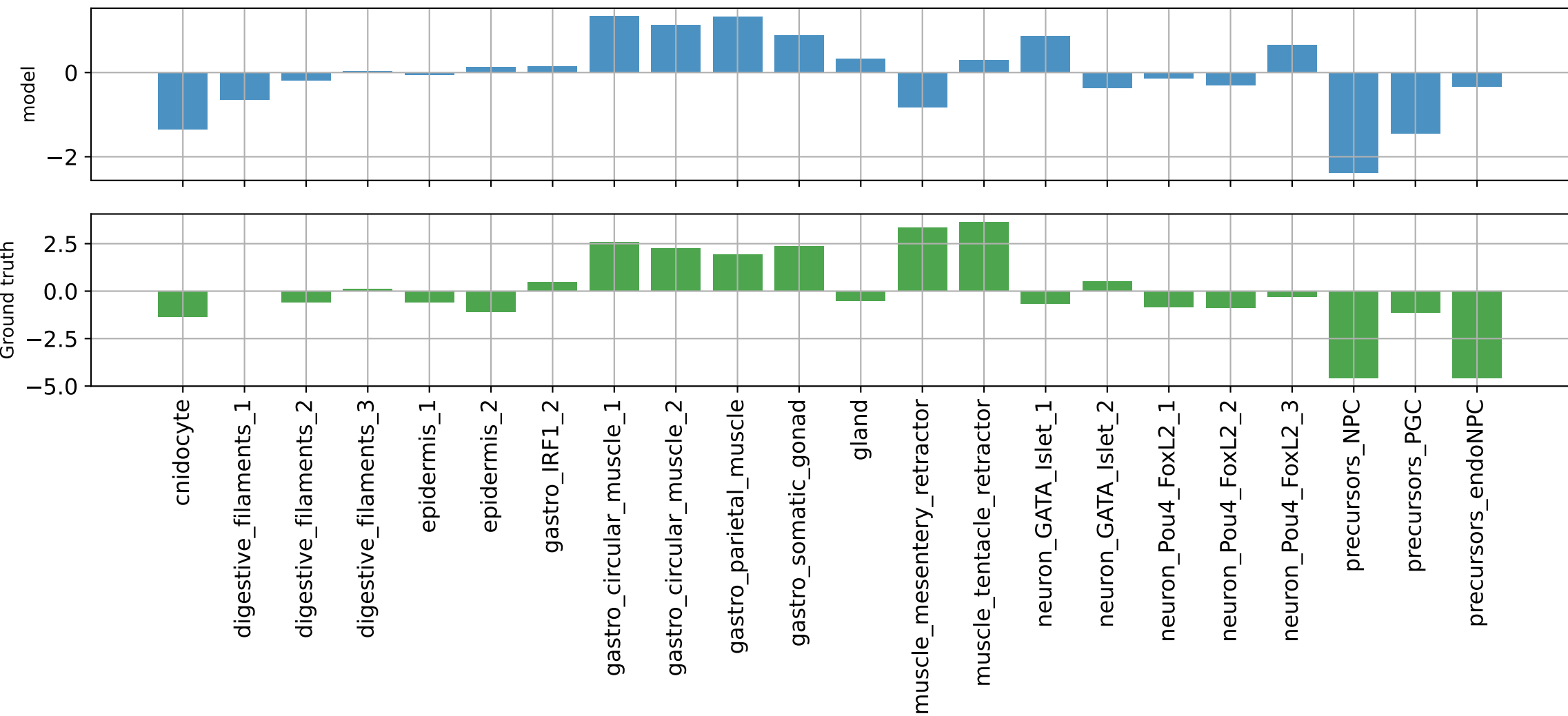
muscle_tentacle_retractor 18: NC_064039.1:5365928-5366428 PCC=0.5827423930168152
