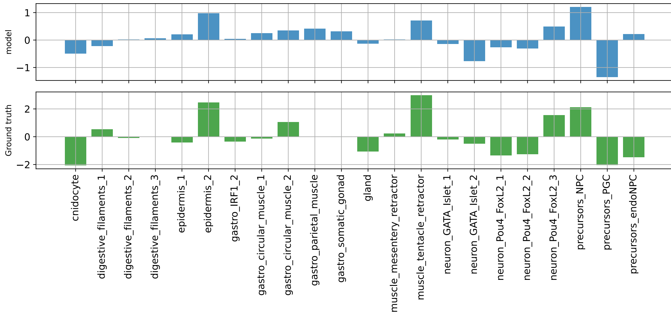
muscle_tentacle_retractor 2: NC_064043.1:4652765-4653265 PCC=0.7996896505355835
