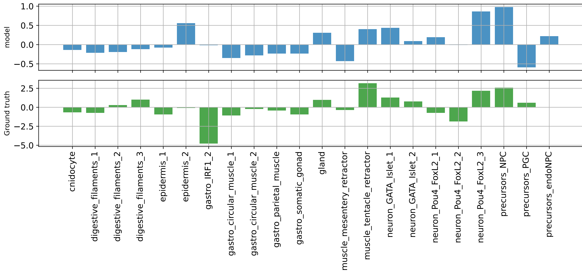
muscle_tentacle_retractor 5: NC_064047.1:2141969-2142469 PCC=0.5129746198654175
