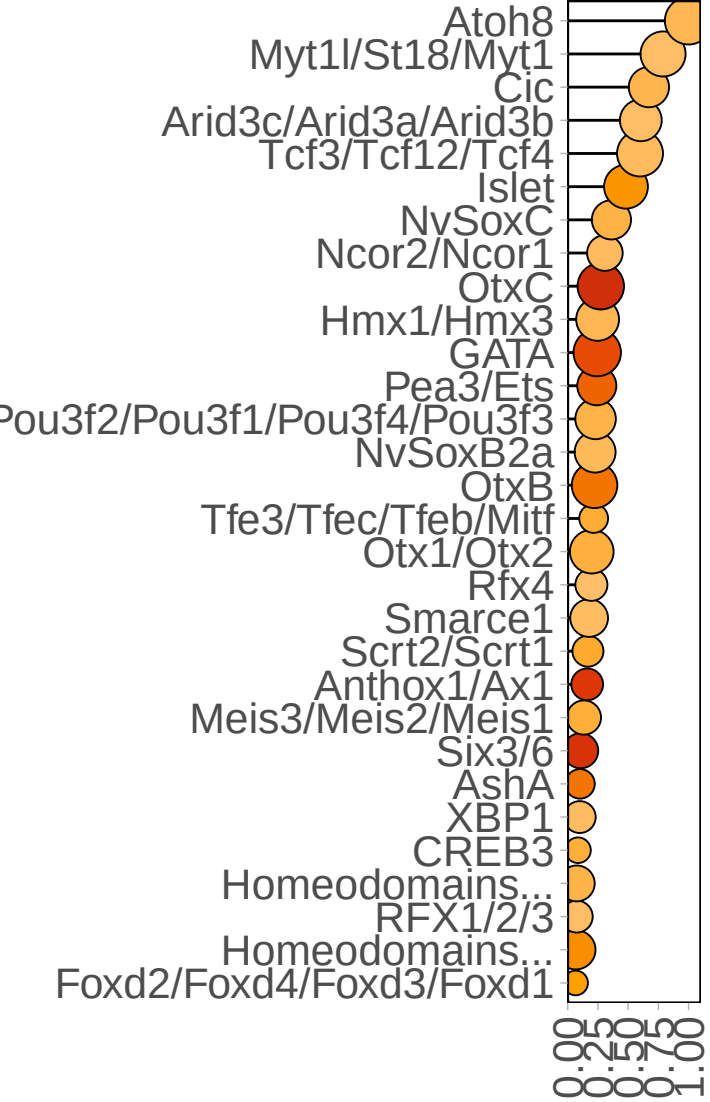
eigenvector centrality
