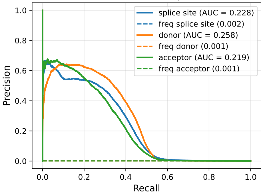
Precision-Recall Curves for Splice Site Classes
