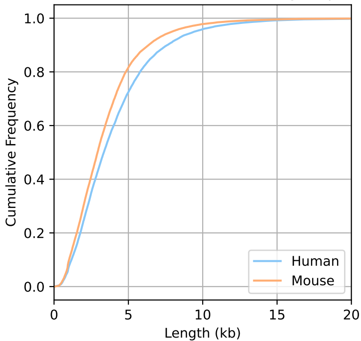
Cumulative Distribution of Summed Exon Lengths per Gene (< 20 kb)
