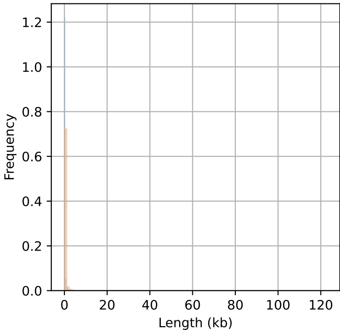
1e6 Distribution of Exon Lengths
