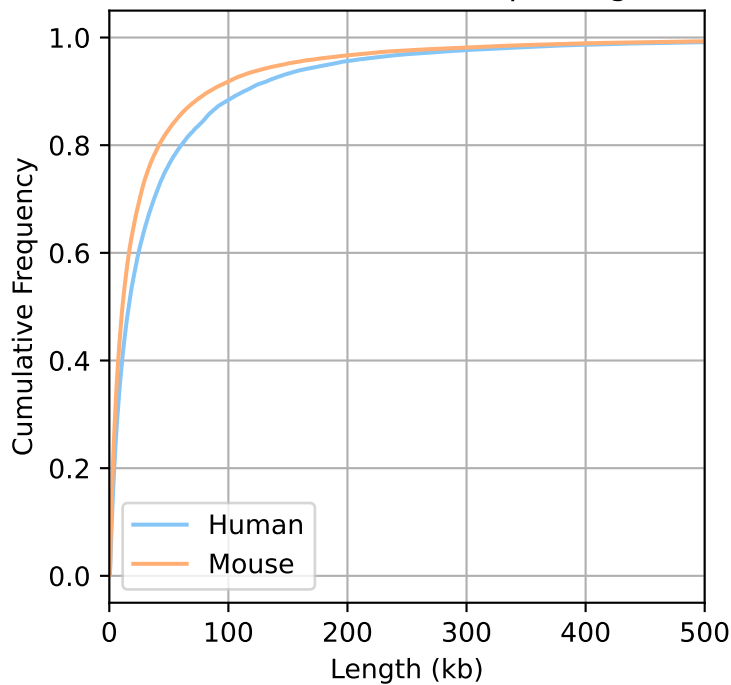
Cumulative Distribution of Transcript Lengths (< 500 kb)
