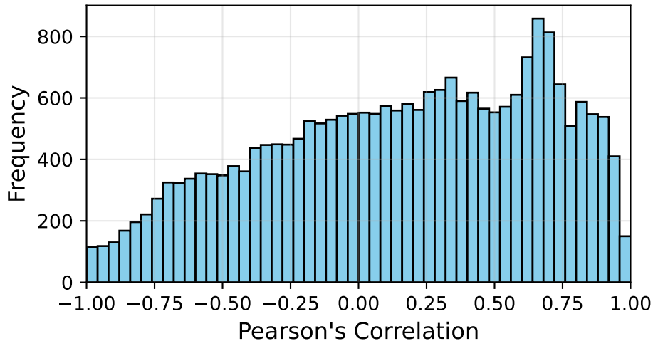
Distribution of Correlations between True and Predicted SSE
