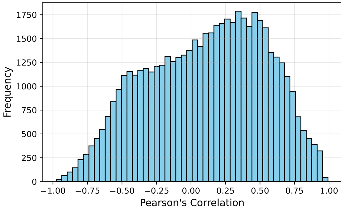
Distribution of Correlations between True and Predicted SSE
