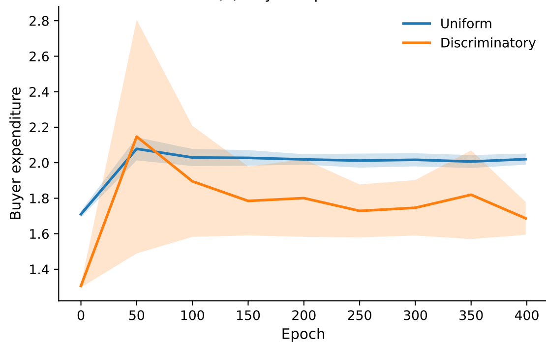
(a) Buyer expenditure
