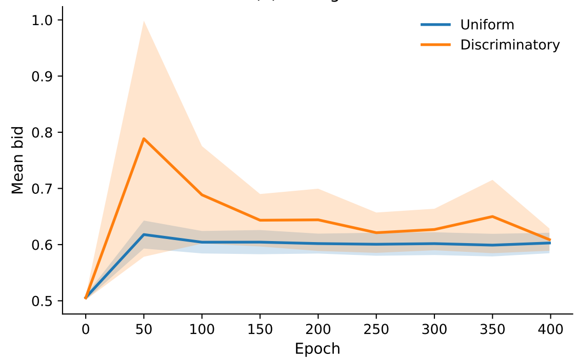
(b) Average bid
