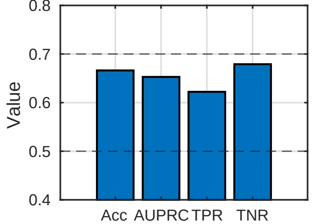
Metrics at Iteration 11 (Max AUPRC)
