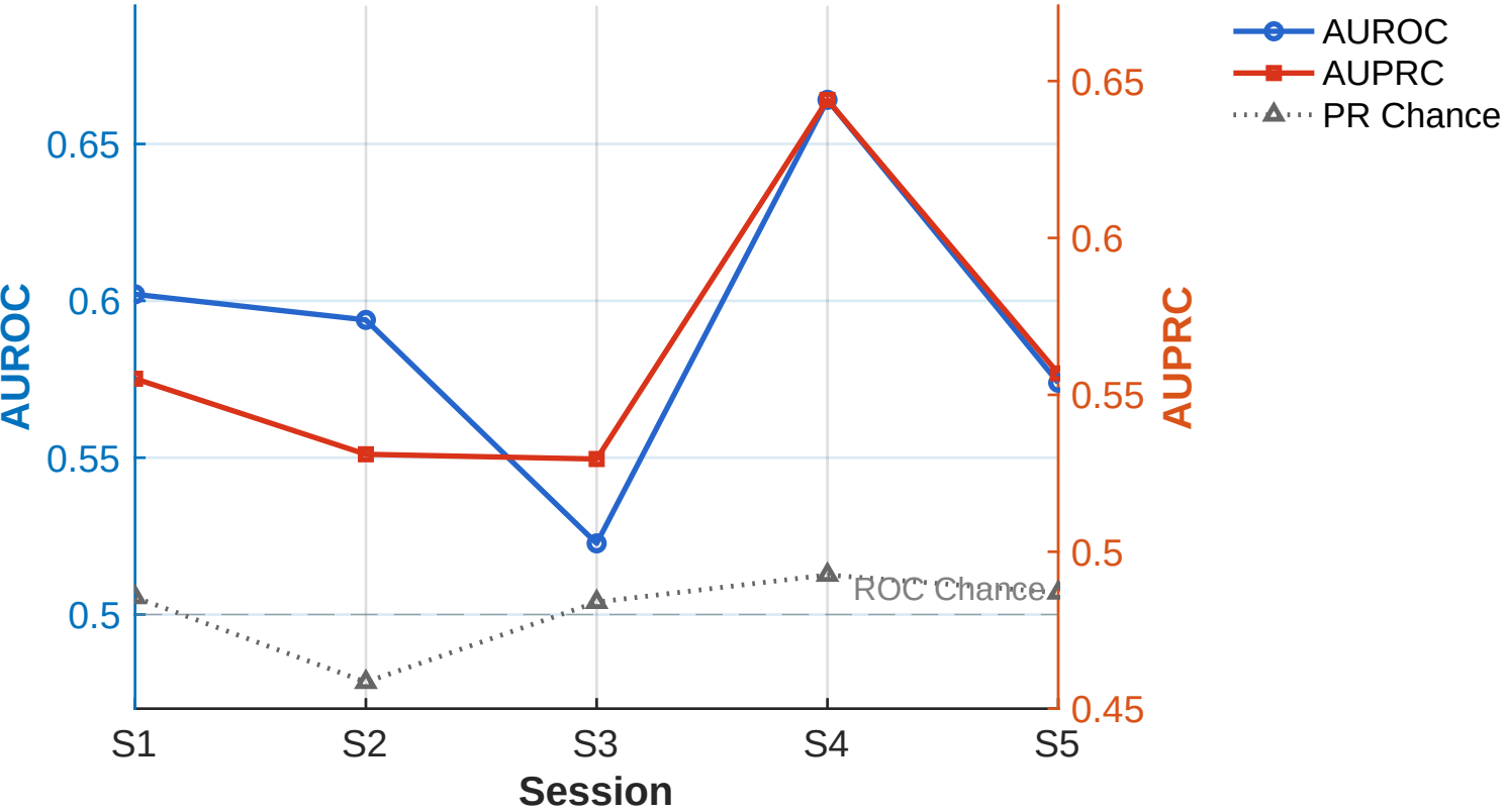
Per-Session AUROC & AUPRC (Ambivalent ignored)
