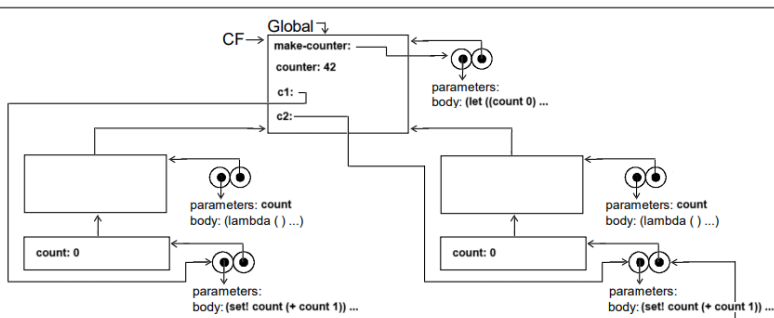
Step13 (define c2 )
