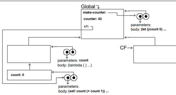
Step9 (define c2 (make-counter))
