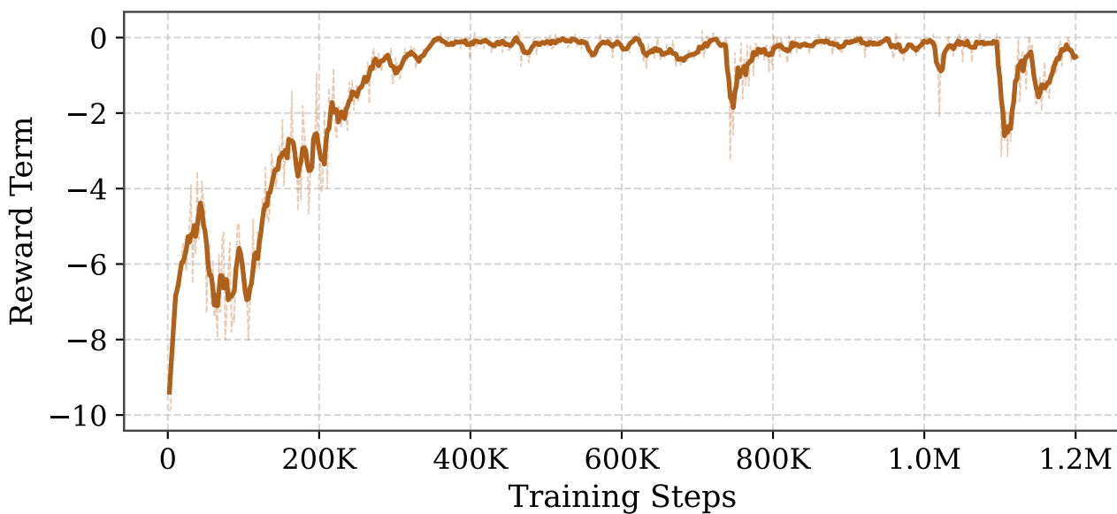
Deadline Penalty
