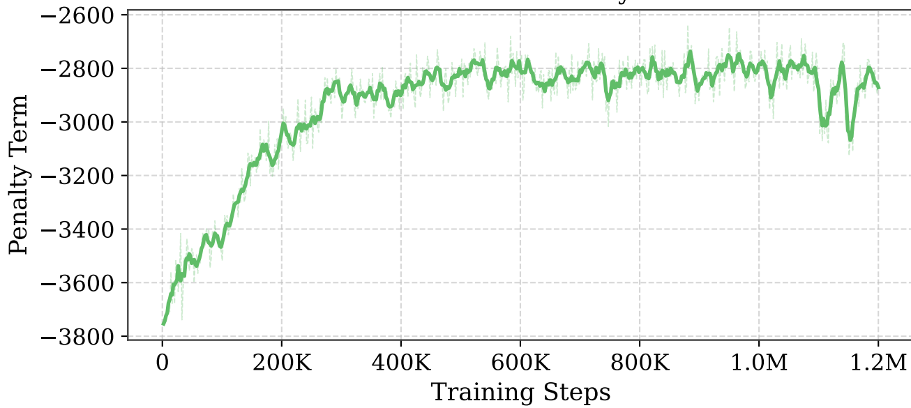
Deadline Penalty
