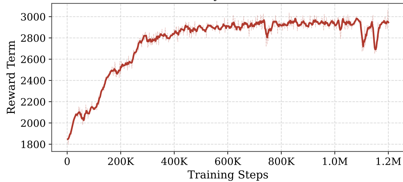
Handover Reward
