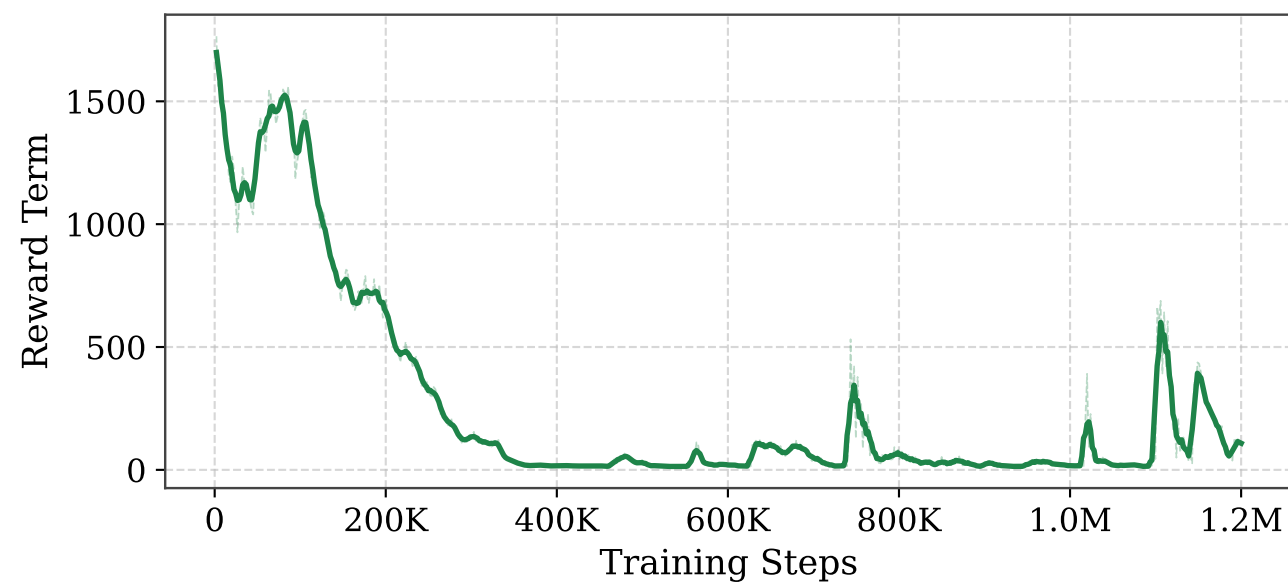
Enqueue Reward
