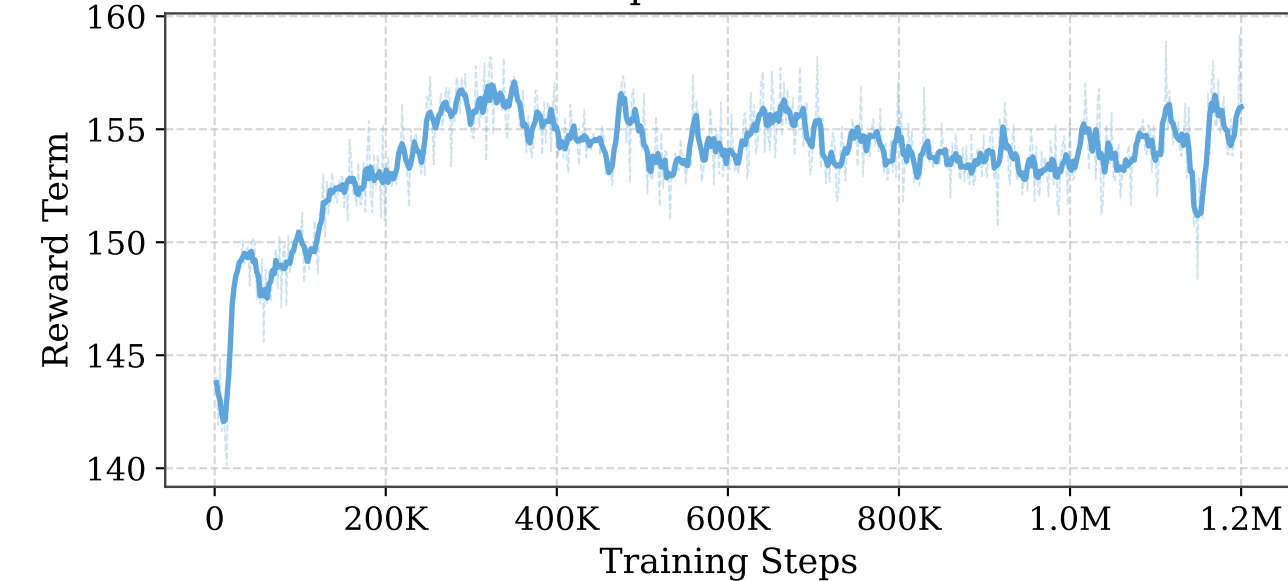
Queue-Full Penalty
