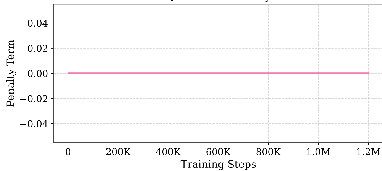
Queue-Full Penalty
