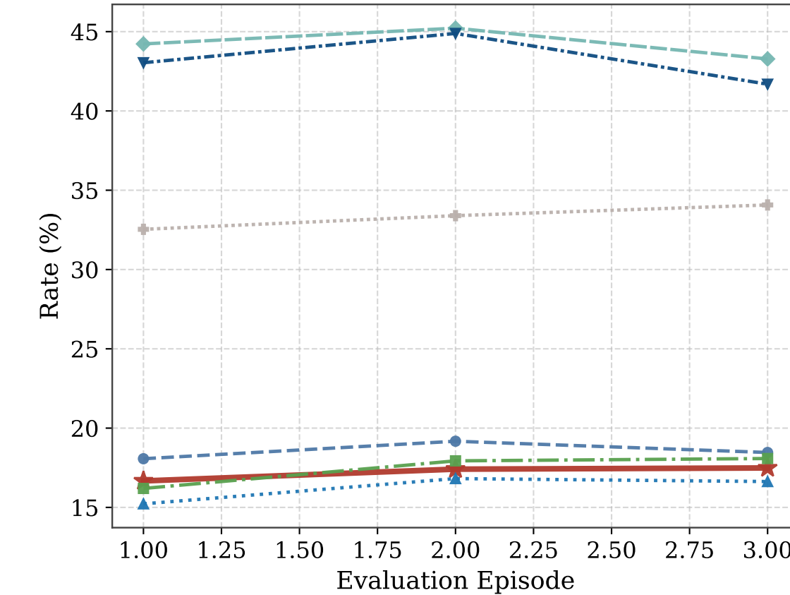
Deadline Violation Rate (Lower is better)
