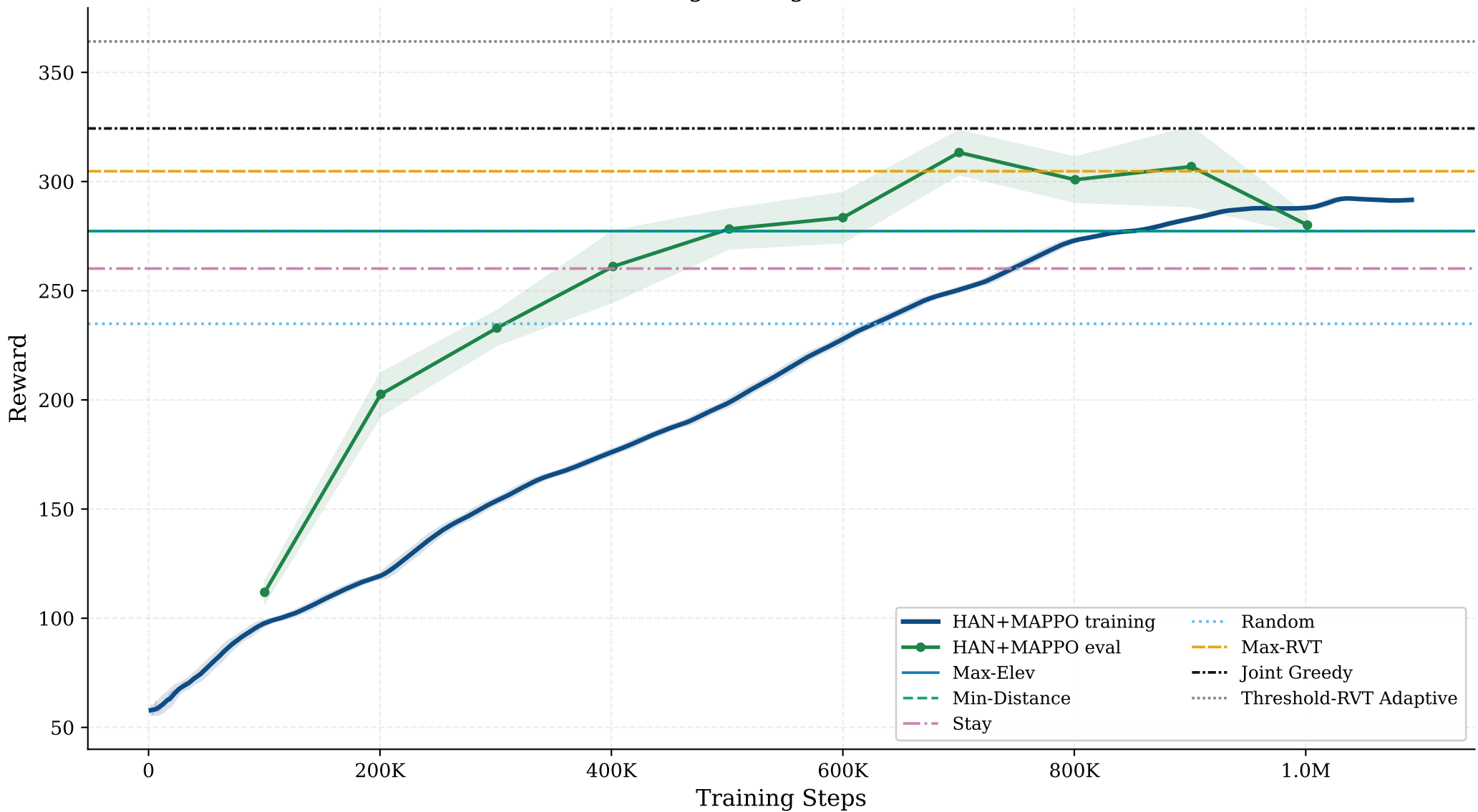
Reward Convergence Against Baseline Levels
