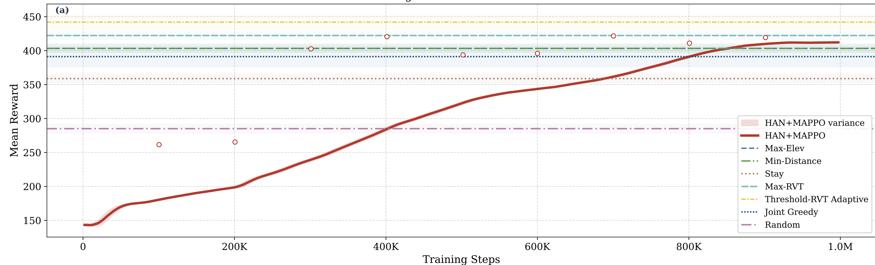
Reward Convergence vs. Heuristic Baseline Levels
